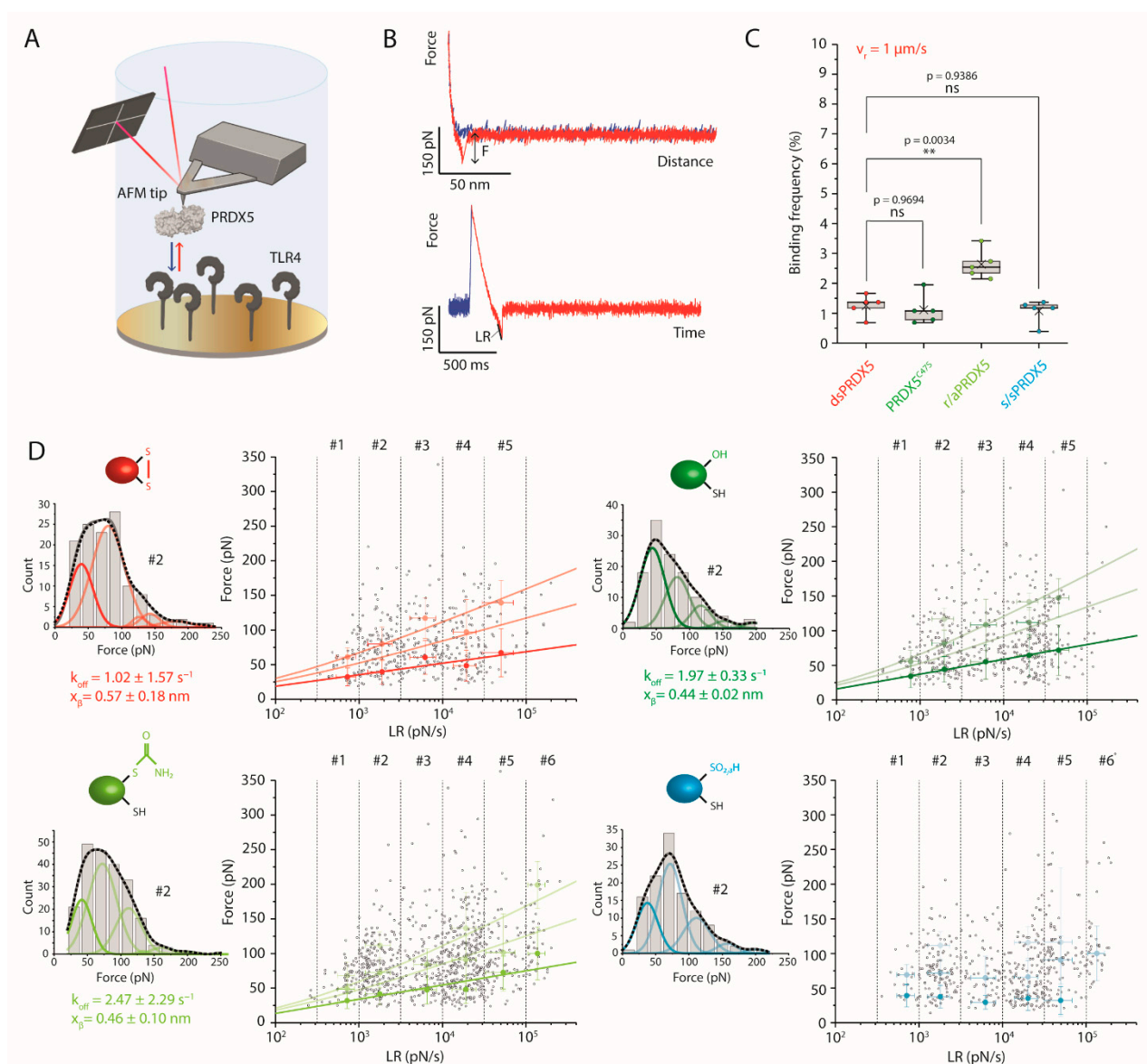
Figure 4. PRDX5 redox forms bind surface-immobilized TLR4 with similar k_{off} . (A) Cartoon showing the experimental set-up used to probe the interaction between the PRDX5 redox forms and TLR4. (B) Representative specific force-distance (FD) and force-time curves. Examples for all redox forms are shown in Supplementary Figure S5. Rupture force ( F ) corresponds to the height of the adhesive peak on the FD curve, and the loading rate (LR) is calculated by fitting the adhesive peak on the force-time curve just before rupture with a linear model. (C) Box plot showing the binding frequencies (BF) obtained at a tip retraction speed of 1 \mu m \cdot s^{-1} . Number of AFM maps, n = 5 for each redox form (dots). Box plot shows mean ( \times ), median ( - ), 25th and 75th percentiles (boxes), and ranges from min to max (whiskers). ns, not significant ( p > 0.05 ). ** p \leq 0.01 (Tukey HSD test). (D) Dynamic force spectroscopy (DFS) analysis for the PRDX5 redox forms. Spectrum of LR was divided into discrete ranges (LR#1–6). For each LR range, a Kernel distribution of the rupture forces (grey line) was generated, as shown on the histogram for LR#2, which allows to determine hidden peaks based on the second derivative. Peaks were fitted with Gaussian functions (colored lines), revealing the most probable rupture forces for single (1st peak) and multiple (following peaks) interactions. These forces were reported on the DFS plot (full colored data points). The Bell-Evans model was fitted to data corresponding to single interactions (solid line), and the predicted rupture forces for two and three simultaneous uncorrelated interactions were calculated using Williams-Evans prediction (dashed lines). From the Bell-Evans model, the k_{off} and x_{\beta} values were extracted. The most probable rupture forces (full colored data points) are peak center \pm S.D.
