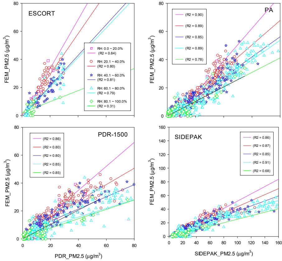
Figure S1. Scatter plots of PM 2.5 concentrations of IRMs with those of FEM, i.e., BAM, by the level of relative humidity. The data points refer to each paired hourly mean value (n=240, except ESCORT which had 120 points due to malfunction of a device with records of high internal temperature values during our outdoor test).
