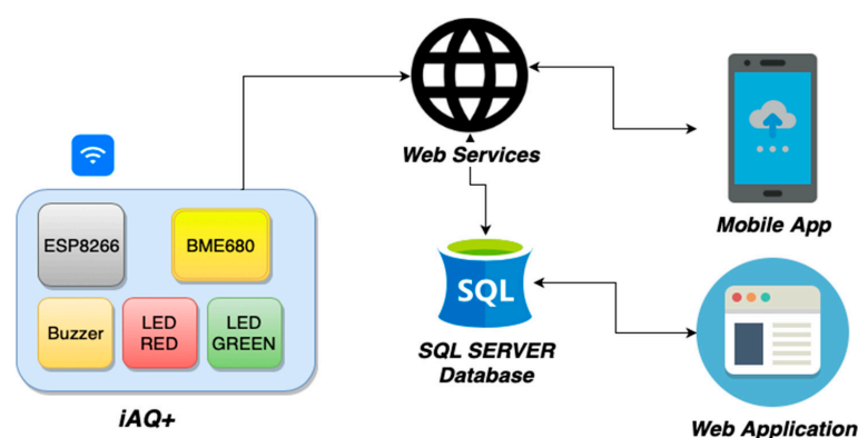
Figure 1. iAQ+ architecture.
