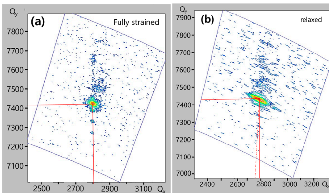
Figure S2. X-ray reciprocal space mapping (RSM) of X-ray diffraction intensity around the (105) reflector for micro LED (a) before and (b) after transfer to Si substrate.
