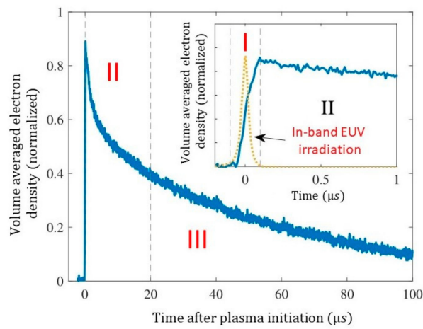
Figure 8. Typical electron density \bar{n}_e in an EUV-induced plasma in H_2 averaged over the measurement geometry. The figure inset is a zoom in up to 1 \mu\text{s} along with the temporally resolved EUV intensity with which the gas is irradiated. The consecutively occurring phases I, II, and III are discussed in the text below. Figure produced using data from [24].
