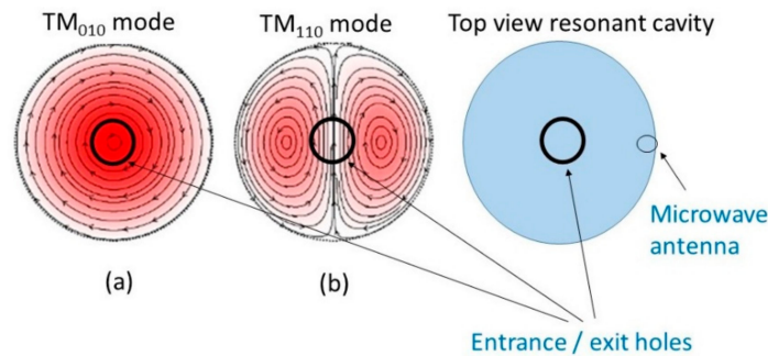
Figure 6. Top view of the electric field distributions of two resonant modes (TM 010 (a) and TM 110 (b)) inside a resonant cavity demonstrating the different local sensitivities. Figure produced using data from [51].
