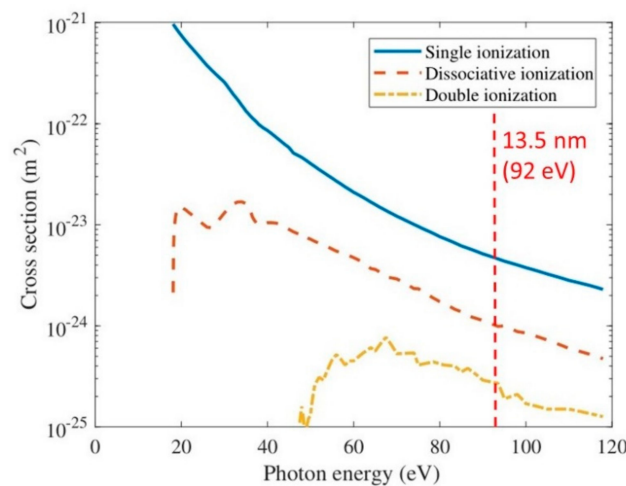
Figure 9. Cross sections for single, dissociative and double photoionization of molecular hydrogen as a function of the photon energy. Figure produced using data from [16,53–55].
