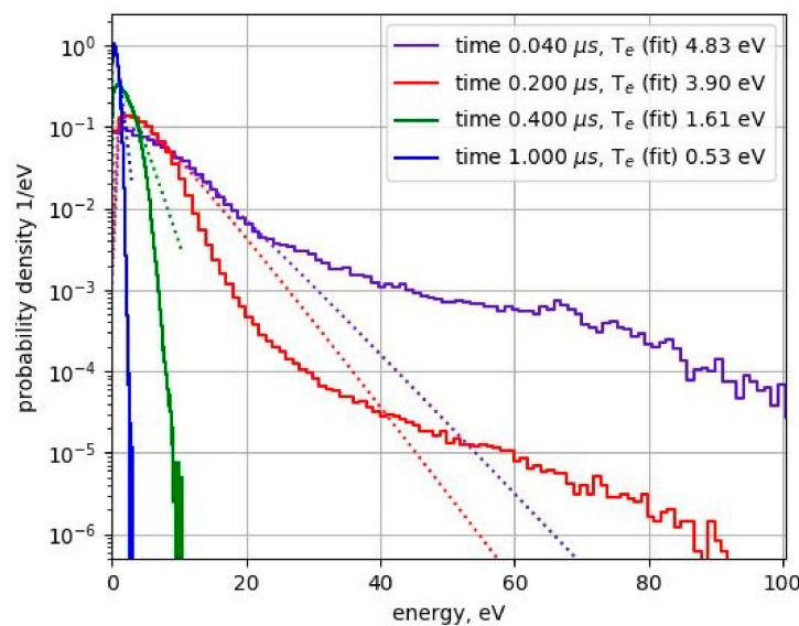
Figure 2. Particle-in-cell simulated electron energy distribution functions (EEDFs) in an EUV-induced plasma during the EUV pulse (purple curve, at t = 0.04 \mu\text{s} the EUV intensity has its maximum value), at the end of the EUV pulse (red curve) and at different moments in time after the EUV pulse ( t = 0.4 \mu\text{s} and t = 1 \mu\text{s} are approximately 0.2 \mu\text{s} and 0.8 \mu\text{s} after the end of the EUV pulse, respectively). The colored dashed-lines represent Maxwellian EEDFs with a temperature corresponding to the calculated mean electron energy.
