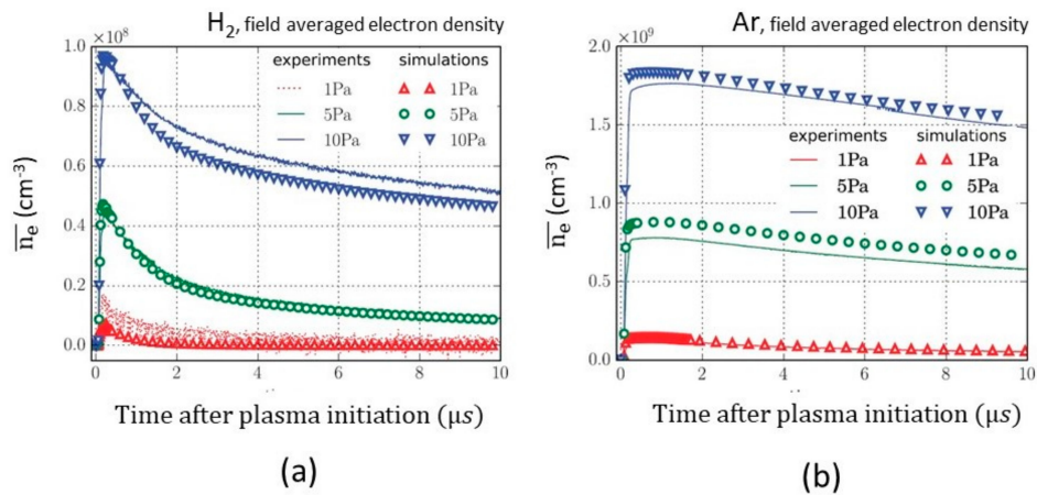
Figure 3. Examples of numerical PIC simulations matching reasonably well measurement of the electron density (measured with Microwave Cavity Resonance Spectroscopy, see next section) in EUV-induced plasmas after irradiation of low pressure hydrogen (a) and argon (b) gas by one single pulse of EUV radiation. Figure produced using data from [21].
