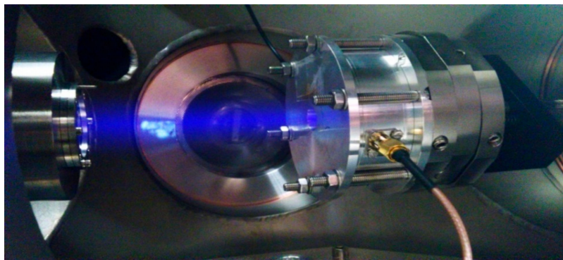
Figure 1. Photograph of the inner side of an experiment chamber in which a low pressure (argon) gas is irradiated with a pulsed beam of Extreme Ultraviolet (EUV) photons. The blueish glow at the position where the EUV beam travels indicates the interaction between the EUV photons and the gas.
