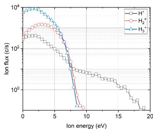
Figure 10. Time-averaged ion energy distribution functions for \text{H}^+ , \text{H}_2^+ , and \text{H}_3^+ ions from an EUV-induced plasma produced in \text{H}_2 gas at 5 Pa. Figure produced using data from [63].
