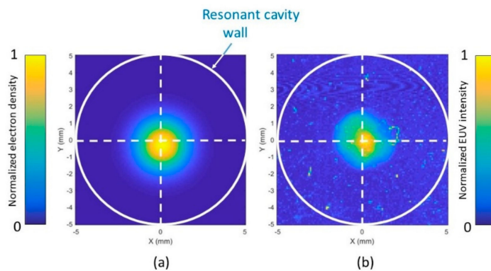
Figure 7. (a) Initial electron density profile—retrieved from multi-mode MCRS measurements—induced by irradiation of a low pressure gas by pulsed EUV radiation (at the maximum intensity of in-band EUV emission from a xenon-based discharge produced plasmas EUV (DPP EUV) source) and (b) an independent measurement of the beam intensity profile at the position of the cavity. False colors are plotted on a linear scale and normalized. Figure produced using data from [51].
