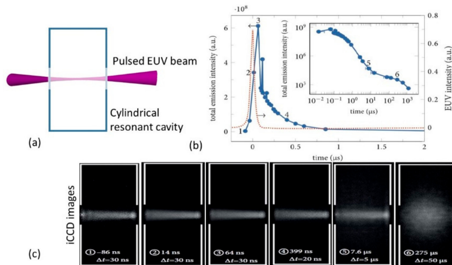
Figure 4. (b) Total emission (in the UV and visible spectrum range) from an EUV-induced plasma in 5 Pa argon created inside a cylindrical measurement volume (a). The numbers displayed in this figure correspond to the numbered images in (c). The horizontal error bars represent the set intensified charge-coupled device (iCCD) camera's gate width. (c) Gated iCCD images at various moments in time (indicated in each picture individually) after one pulse of EUV-irradiation. The beam of EUV photons is directed through a cylindrical aluminum measurement chamber from the left to the right (the side walls are indicated with white lines). The side walls of the measurement chamber are made of a mesh for visibility and the top and bottom lids contain concentric holes for entrance and exit of the EUV beam. \Delta t indicates the used gate width of the camera. Intensities are normalized for each image individually. Figure produced using data from [26].
