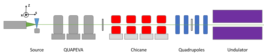
Figure 1. COXINEL transport line scheme. Left to right: Laser pulse focused on a gas jet (blue), triplet of QUAPEVAs (grey), first screen for electron beam profile measurement (white), chicane (red), a second set of electro-magnetic quadrupoles (blue), screen before and after the undulator (white), and cryo-ready undulator (purple).
