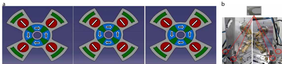
Figure 3. (a) QUAPEVA magnetic design with different orientation of the cylindrical magnets: maximum (left), intermediate (middle), minimum gradient (right). (b) Mechanical shims applied to one of the QUAPEVAs to compensate for the skew terms.
