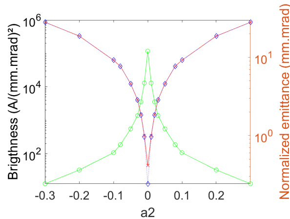
Figure 14. Brightness (●) of the electron beam at the center of the undulator versus QUAPEVA 2 a_2 skew term and horizontal (x) and vertical (◆) normalized emittance in log scale. Simulation using a “monochromatic” 176 \pm 0.1 MeV beam with \sigma'_{z,i} = 2 mrad and \sigma'_{x,i} = 3.12 mrad, a charge of 0.1 \pm 0.02 pC, \epsilon_{z,i}, \epsilon_{x,i} = 0.2 mm.mrad, transported with the “slit-undulator” optics and the slit in the chicane open to 3.2 mm.
