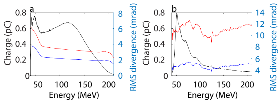
Figure 2. Initial beam electron distribution (black), vertical (blue), and horizontal (red) divergence. (a) Low divergence beam (average over a set of 20 distributions), (b) high divergence beam (single-shot).
