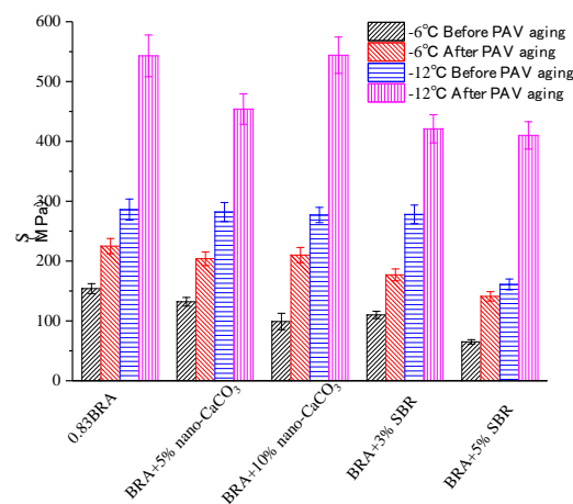
Figure 6. Creep stiffness S of nano- \text{CaCO}_3 /BRA and SBR/BRA compound-modified asphalt before and after pressure aging vessel (PAV) aging.
