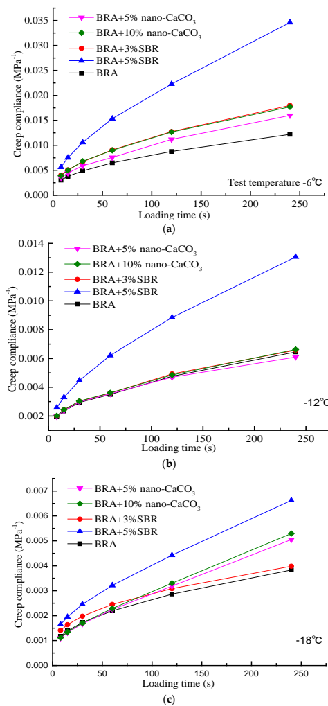
Figure 9. Creep compliance curve of different compound-modified asphalts: (a) the curves of creep compliance of BRA compound-modified asphalt in -6^{\circ}\text{C} ; (b) the curves of creep compliance of BRA compound-modified asphalt in -12^{\circ}\text{C} ; (c) the curves of creep compliance of BRA compound-modified asphalt in -18^{\circ}\text{C} .
