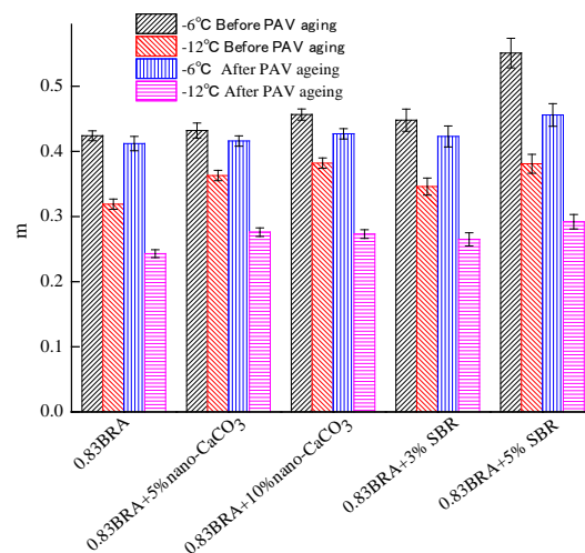
Figure 7. m value of nano- \text{CaCO}_3 /BRA and SBR/BRA compound-modified asphalt before and after pressure aging vessel (PAV) aging.
