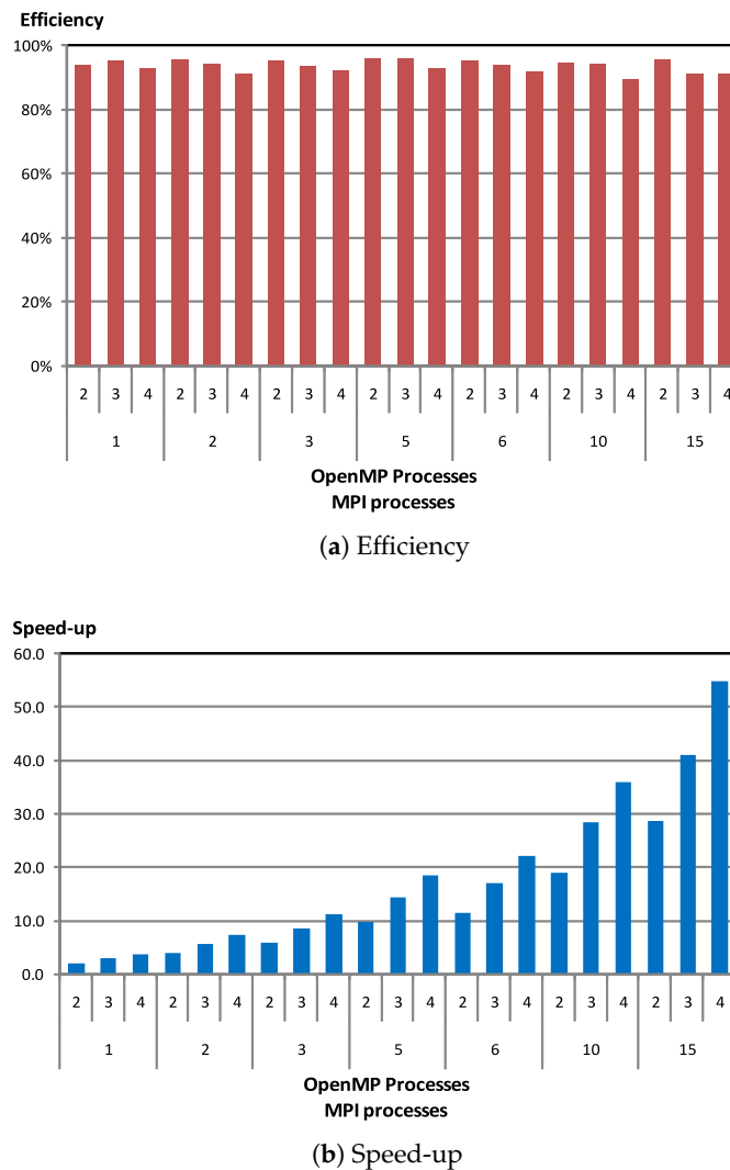
Figure 5. Hybrid parallel Jaya algorithm. Iterations = 30,000. Population = 256. Runs = 30. (a) Efficiency of the parallel algorithm. (b) Speed-up with respect to the sequential execution.
