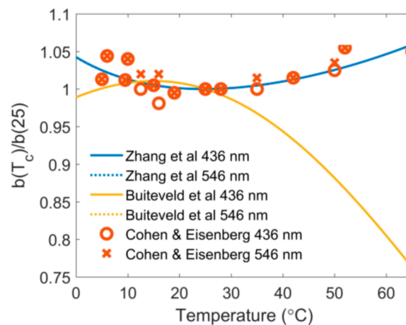
Figure 1. The temperature variations of light scattering by pure water, calculated using the Zhang and Hu [9] model (i.e., Equation (2)) at 436 and 546 nm and normalized by their respective values at 25 °C, are compared with the estimates using the Buiteveld, et al. [7] model and with the measurements by Cohen and Eisenberg [6]. Note that the normalized variations estimated by the Zhang and Hu model overlap with each other at the two wavelengths.
