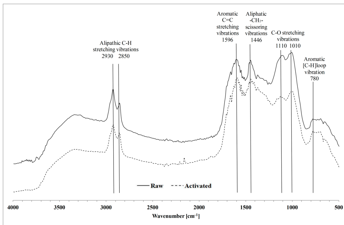
Figure 2. FTIR-PAS spectra of raw and activated hydrochar.
