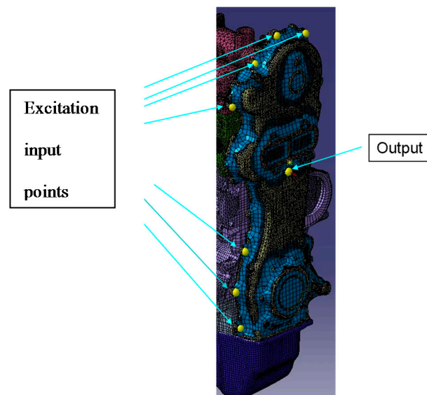
Figure 6. Vibro-acoustic model for the vibration analysis.
