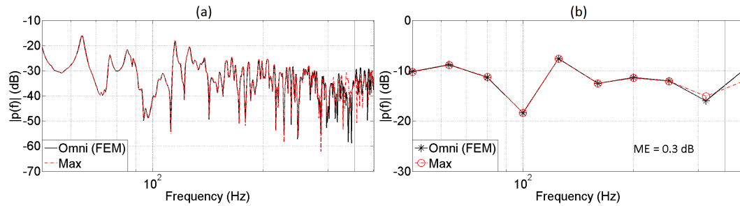
Figure 21. Comparison of full (a) and 1/3 octave band (b) frequency responses. Translated PWE and omnidirectional room impulse response (FEM) at translated Position 2.
