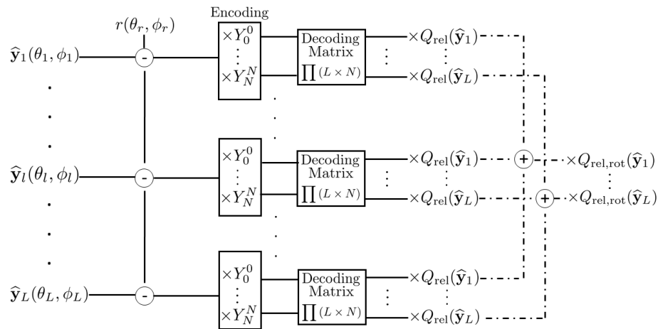
Figure 17. Rotation scheme.
