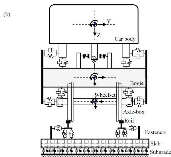
Figure 1. Coupling dynamic model of a metro vehicle and a conventional ballastless track: (a) Elevation; (b) End view.
