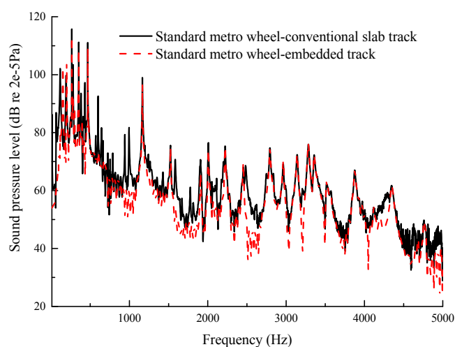
Figure 16. Total SPLs considering standard metro wheels coupled with the conventional slab track and embedded track (simulation results).
