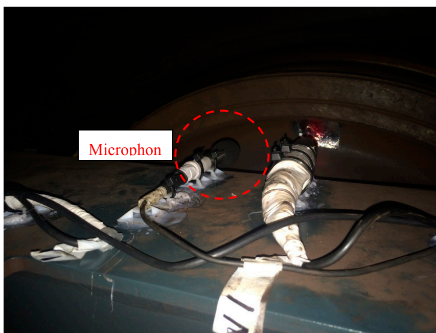
Figure 11. Microphone arrangement.
