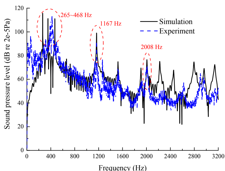
Figure 12. Comparison between simulation and experimental results of SPL of the leading wheel.
