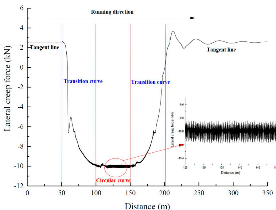
Figure 7. Lateral creep force of the leading wheelset when a vehicle negotiates a narrow curve (simulation results).
