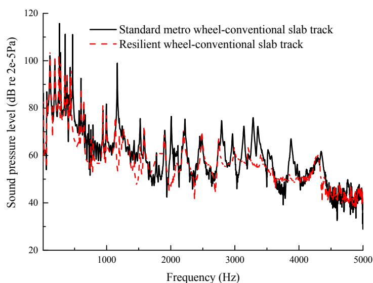
Figure 19. SPLs of common slab track coupled with the standard metro wheel and elastic wheel (simulation results).
