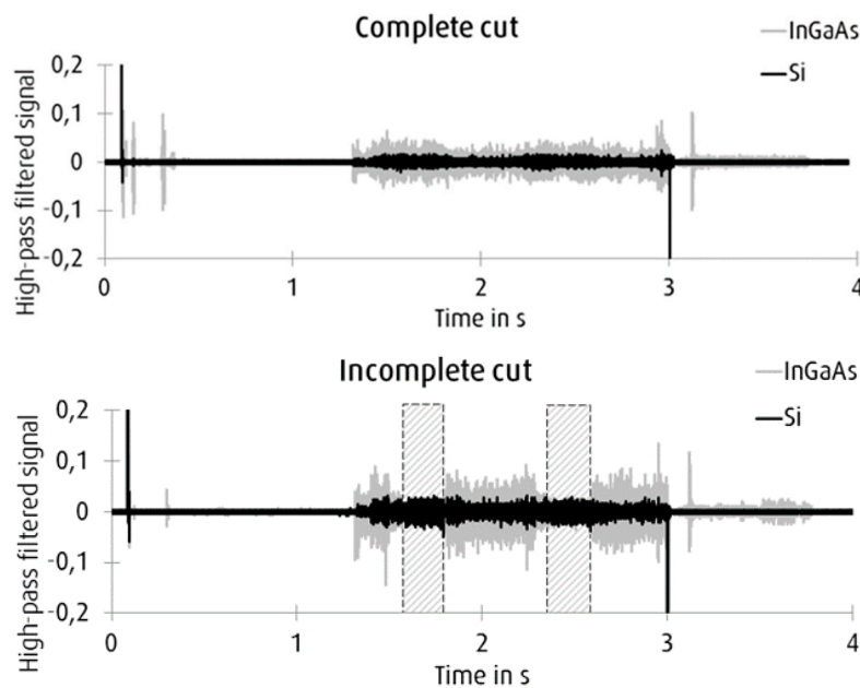
Figure 5. High pass filtered signal of a complete ( top ) and incomplete cut ( bottom ). The time domain in which the cutting interruption occurs is marked by the two grey shaded rectangular with dashed lines.
