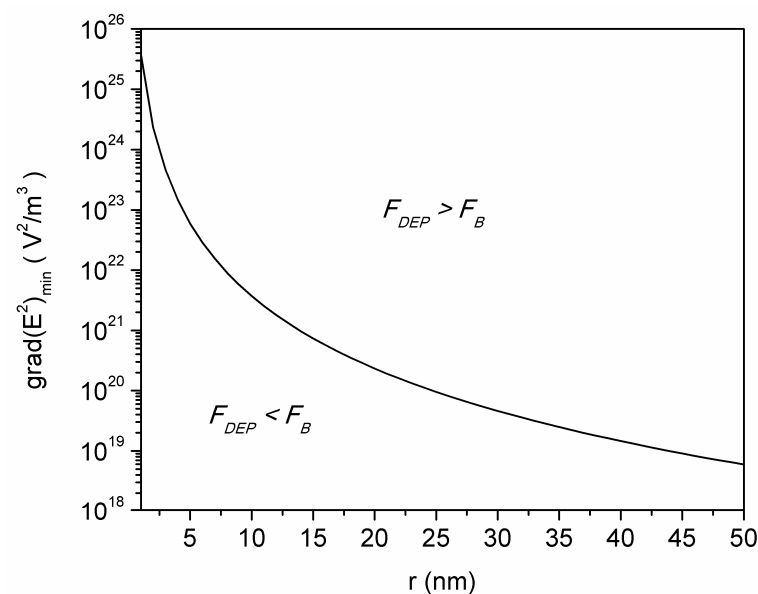
Figure 2. The theoretical dependence of (\nabla E^2)_{\min} on the radius of a manganese ferrite particle in kerosene.
