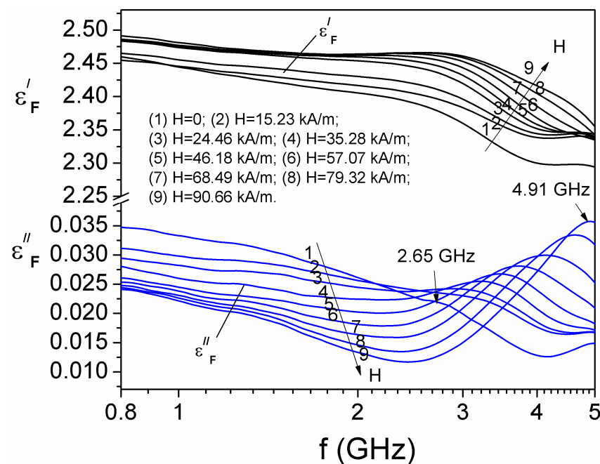
Figure 3. The frequency dependence of the components of the complex dielectric permittivity at different values, H , of the magnetic field.
