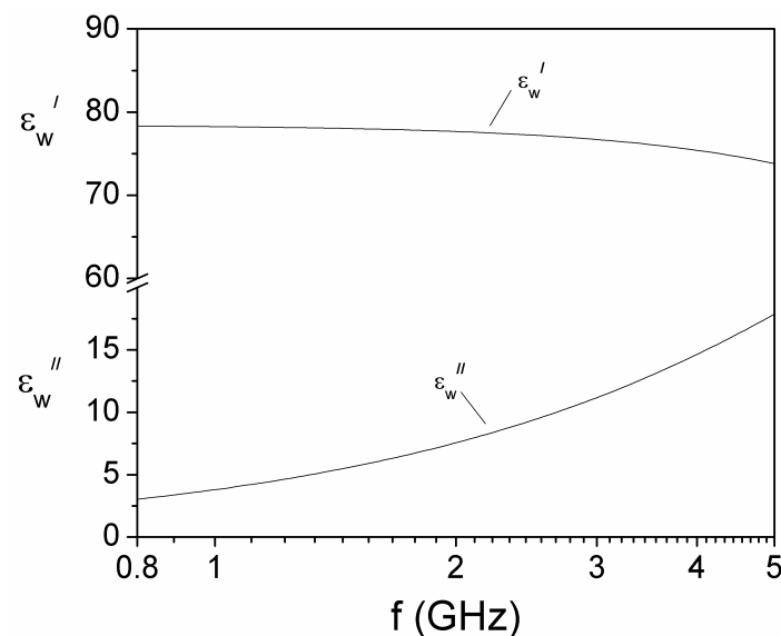
Figure 7. Frequency dependence of the components of the complex dielectric permittivity of distilled water.
