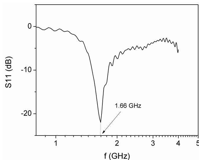
Figure 10. Frequency dependence of the reflection coefficient of the cable-antenna system.
