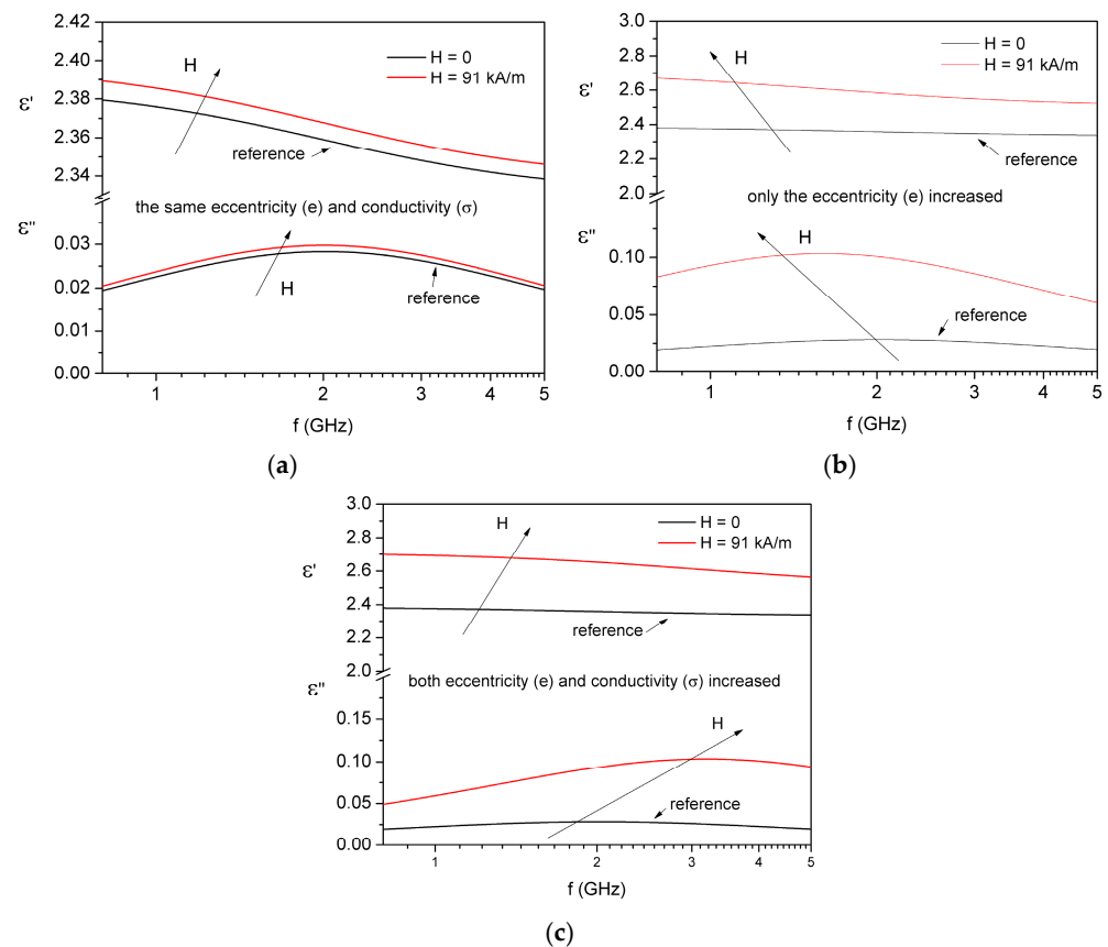
Figure 4. Frequency and magnetic field theoretical dependencies of the complex dielectric permittivity of a ferrofluid. (a) The effect of the magnetic field, assuming no particle aggregation; (b) the effect of small particle aggregation under the magnetic field; and (c) the effect of particle aggregation and conductivity change by magnetoresistive tunneling.
