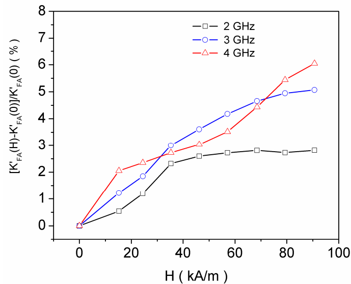
Figure 6. The relative variation in the real component of the Clausius–Mossotti factor of ferrofluid in air ( K'_{FA} ) as a function of the magnetic field ( H ).
