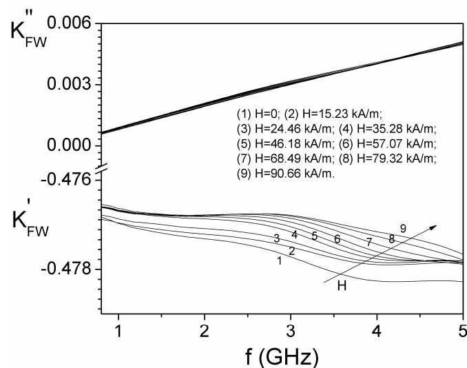
Figure 8. Frequency dependence of the components ( K'_{FW} ) and ( K''_{FW} ) of the Clausius–Mossotti complex factor of the ferrofluid sample in distilled water for different values, H , of the magnetic field.
