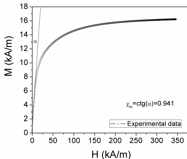
Figure 1. The magnetization curve of the investigated ferrofluid sample.
