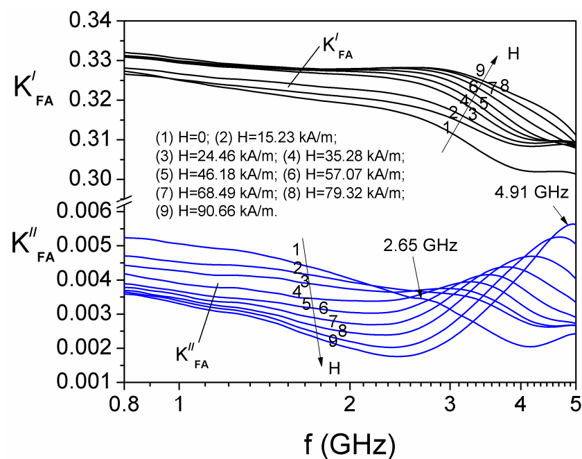
Figure 5. Frequency dependence of the components ( K'_{FA} ) and ( K''_{FA} ) of the Clausius–Mossotti complex factor of the ferrofluid sample in air for different values, H , of the magnetic field.
