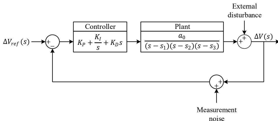
Figure 2. Closed-loop PID-based vehicle cruise control system with external disturbance and measurement noise.
