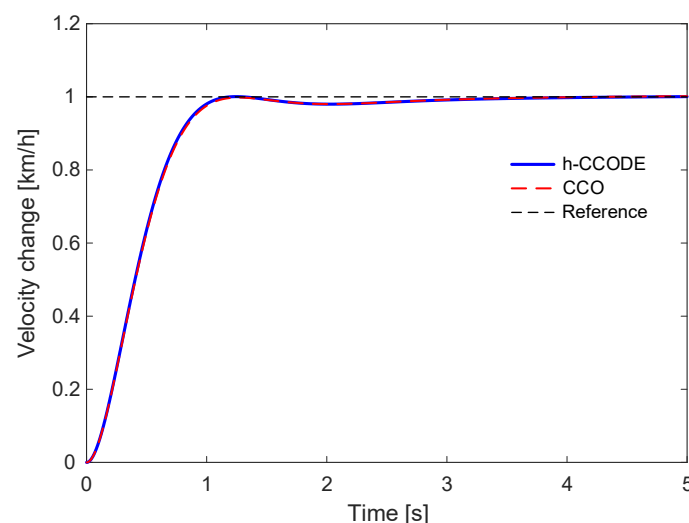
Figure 4. Closed-loop step responses of the cruise control system using h-CCODE and CCO.
