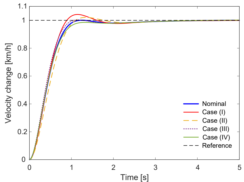
Figure 10. Closed-loop responses of the proposed controller under nominal and uncertain system parameters.
