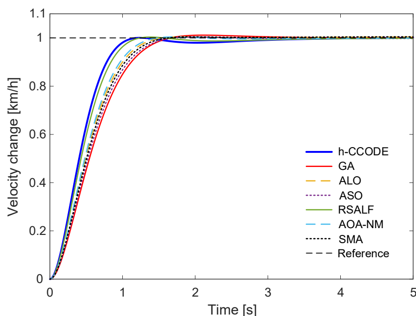
Figure 5. Closed-loop responses of the proposed method and existing optimization-based controllers.
