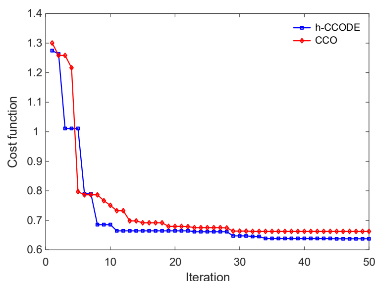
Figure 3. Convergence curves of the cost function for h-CCODE and CCO.
