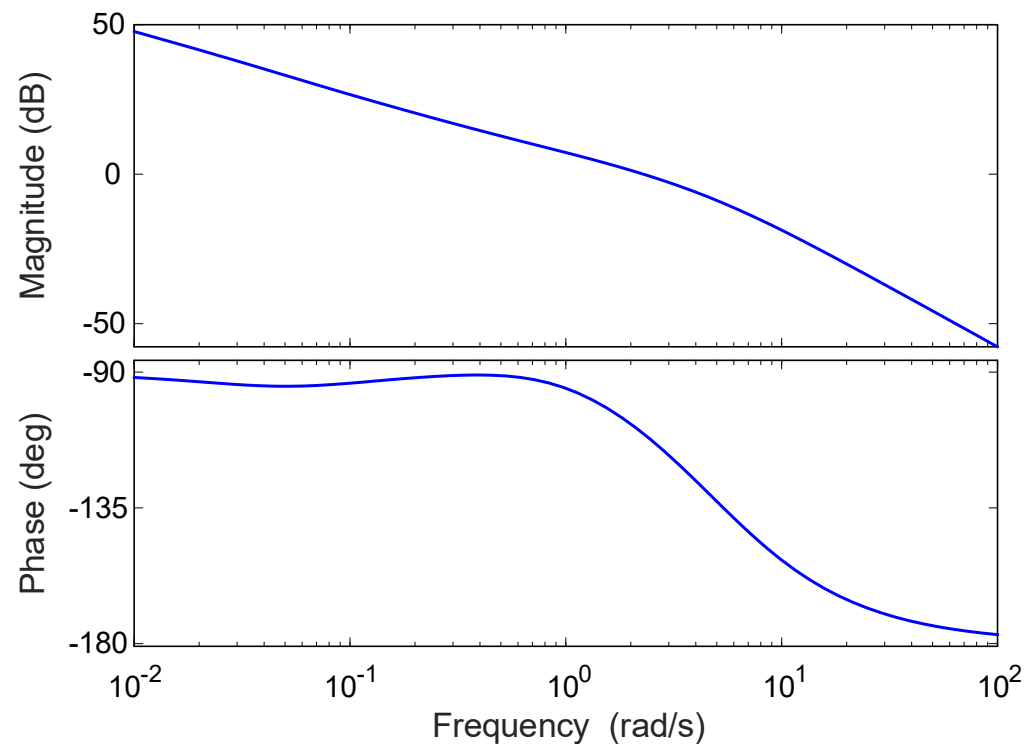
Figure 8. Open-loop Bode diagram of the h-CCODE-tuned PID-controlled cruise control system.
