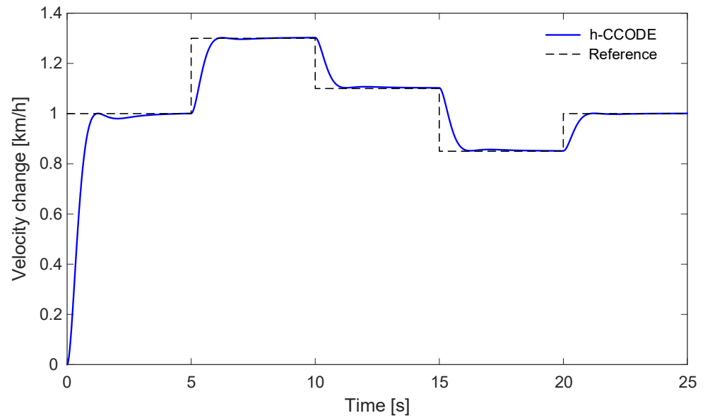
Figure 9. Reference tracking performance of the proposed controller under successive positive and negative speed variations.
