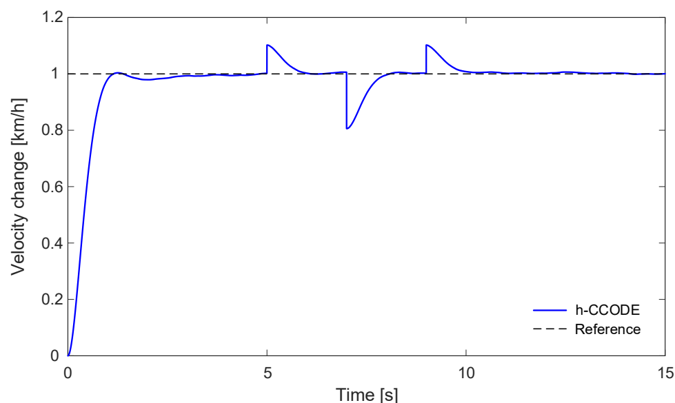
Figure 7. Disturbance rejection performance of the proposed h-CCODE-based PID controller.
