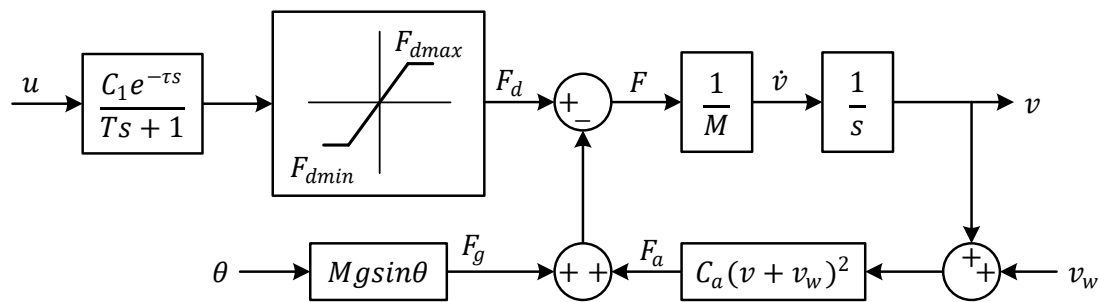
Figure 1. Nonlinear vehicle cruise control model with actuator, aerodynamic drag, and road-slope effects.
