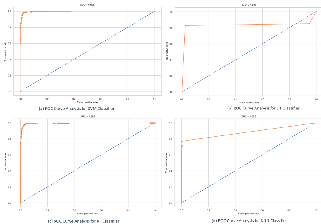
Figure 7. ROC for each Classifier.
