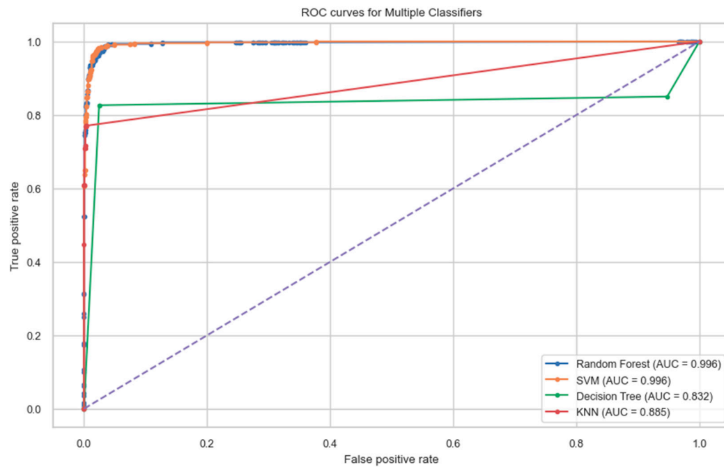
Figure 8. Comparison of ROC Curves for all Classifiers.
