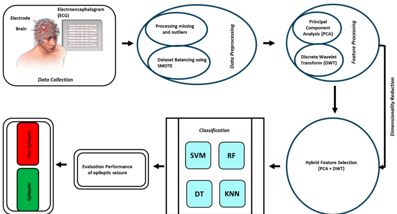
Figure 2. Proposed Epileptic Seizures Detection Model.
