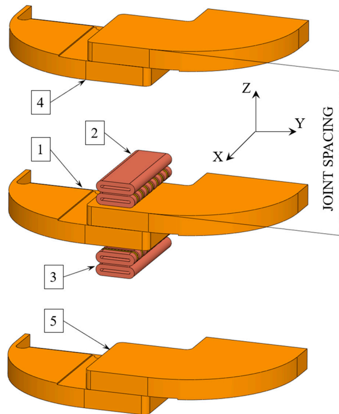
Figure 7. Model of ECP, TO, and adjacent solder joints: 1—TO; 2—upper element of ECP; 3—lower element of ECP; 4—upper solder joint; 5—lower solder joint.
