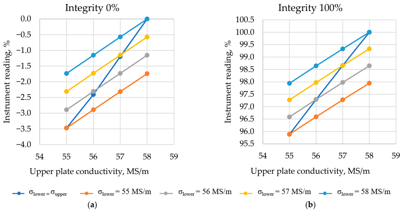
Figure 12. Correlation between the instrument readings and the electrical conductivity of the TO: (a) correlation for TO with 0% soldering integrity; (b) correlation for TO with 100% soldering integrity.
