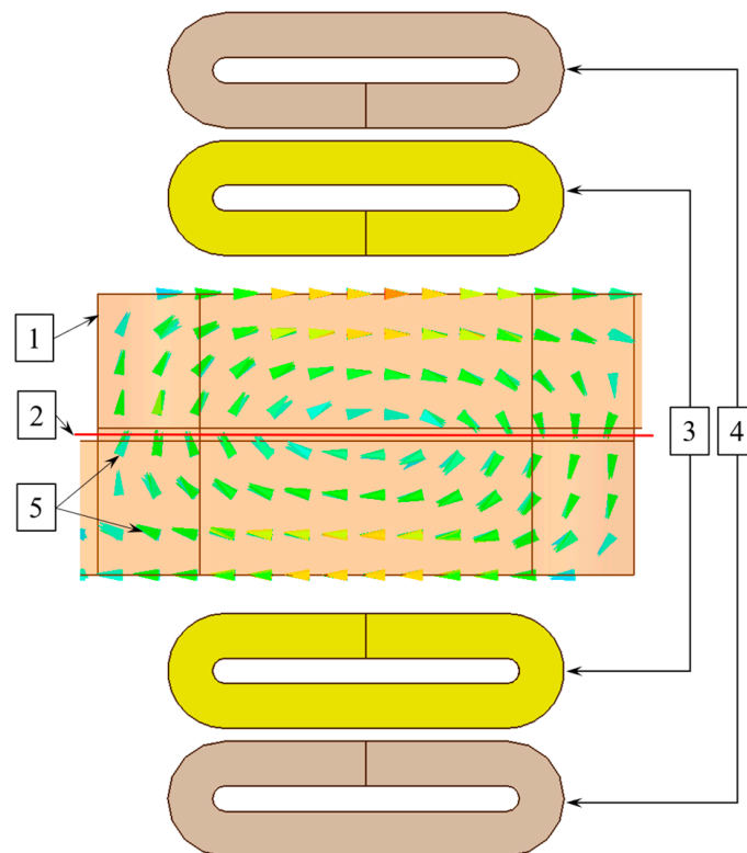
Figure 8. Pattern of eddy current lines in the finite element model of the TO: 1—TO; 2—plane of soldered lap joint; 3—excitation coils; 4—shielding coils; 5—eddy current lines.
