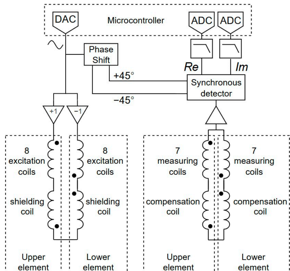
Figure 5. Electrical schematic diagram of ECP [4].
