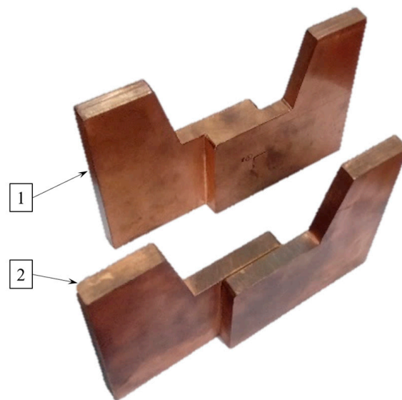
Figure 11. Reference blocks of soldered lap joints: 1—RB of 100% soldering integrity; 2—RB of 0% soldering integrity.
