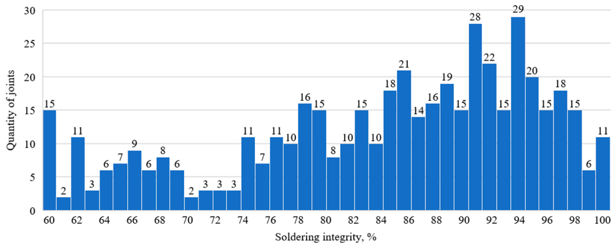
Figure 13. Statistics of measurements of soldering integrity of soldered lap joints in TVF-60-2 turbine generator.
