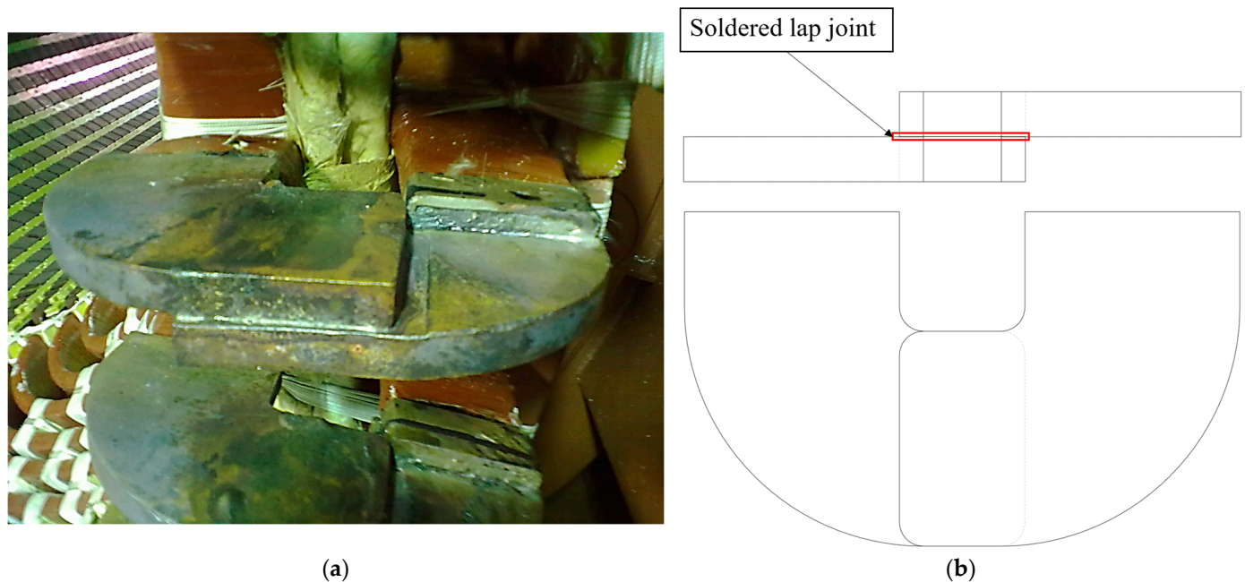
Figure 1. Solder joint of copper busbars: (a) photograph of TO in stator winding; (b) drawing of TO [4].
