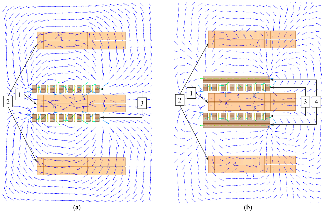
Figure 6. Magnetic field pattern of the finite element model of an ECP (a) without shielding coils and (b) with shielding coils: 1—TO; 2—adjacent solder joints; 3—excitation coils; 4—shielding coils.
