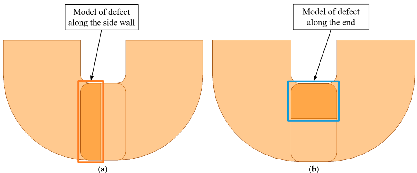
Figure 3. Models of defect simulators: (a)—TO with a model of a soldering defect along the side wall; (b)—TO with a model of a soldering defect along the end.
