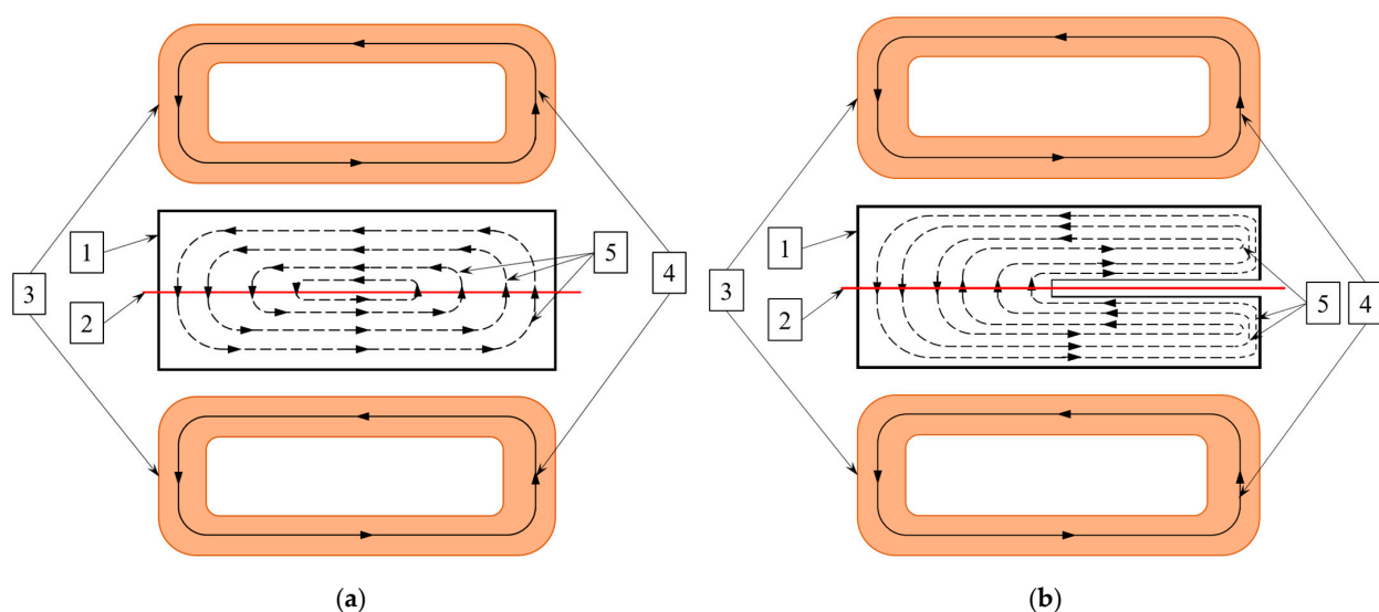
Figure 2. Vector field of propagation of eddy currents in two-element tangential ECP in (a) TO without defects and (b) TO with defects: 1—TO; 2—defect location plane; 3—tangentially placed ECP coils; 4—current direction in ECP coils; 5—eddy current propagation lines in TO.
