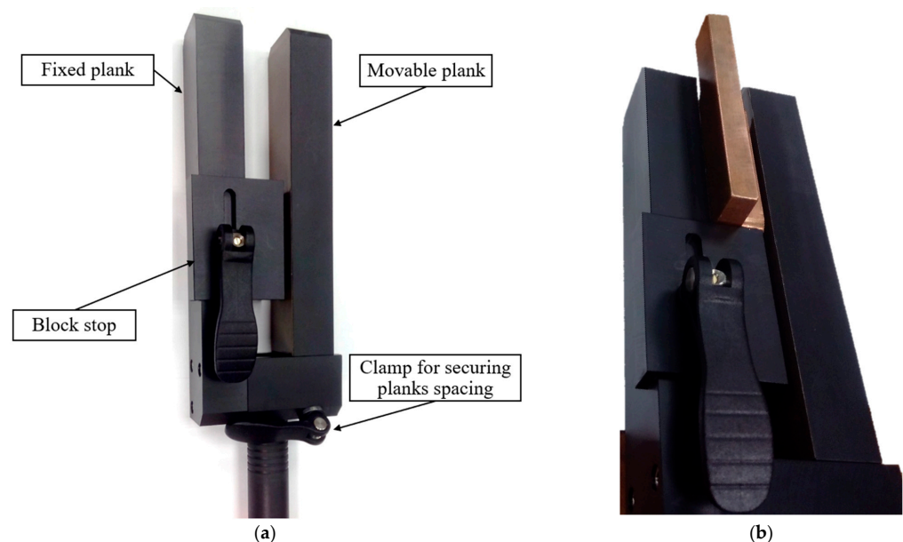
Figure 10. Photographs of the developed ECP: (a)—ECP design; (b)—ECP installation on RB [4].
