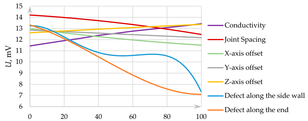
Figure 9. Correlations of ECP model signal with deviations in studied parameters.
