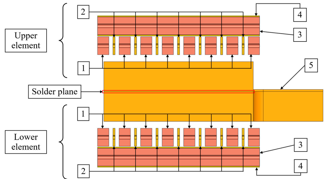
Figure 4. Close-up of ECP coils and TO: 1—excitation coils; 2—measuring coils; 3—shielding coils; 4—compensation coils; 5—TO [4].
