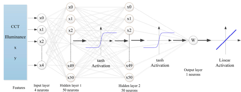
Figure 9. Architecture of whiteness prediction model.
