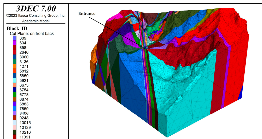
Figure 11. Three-dimensional model employed for numerical analysis in 3DEC v.7.
