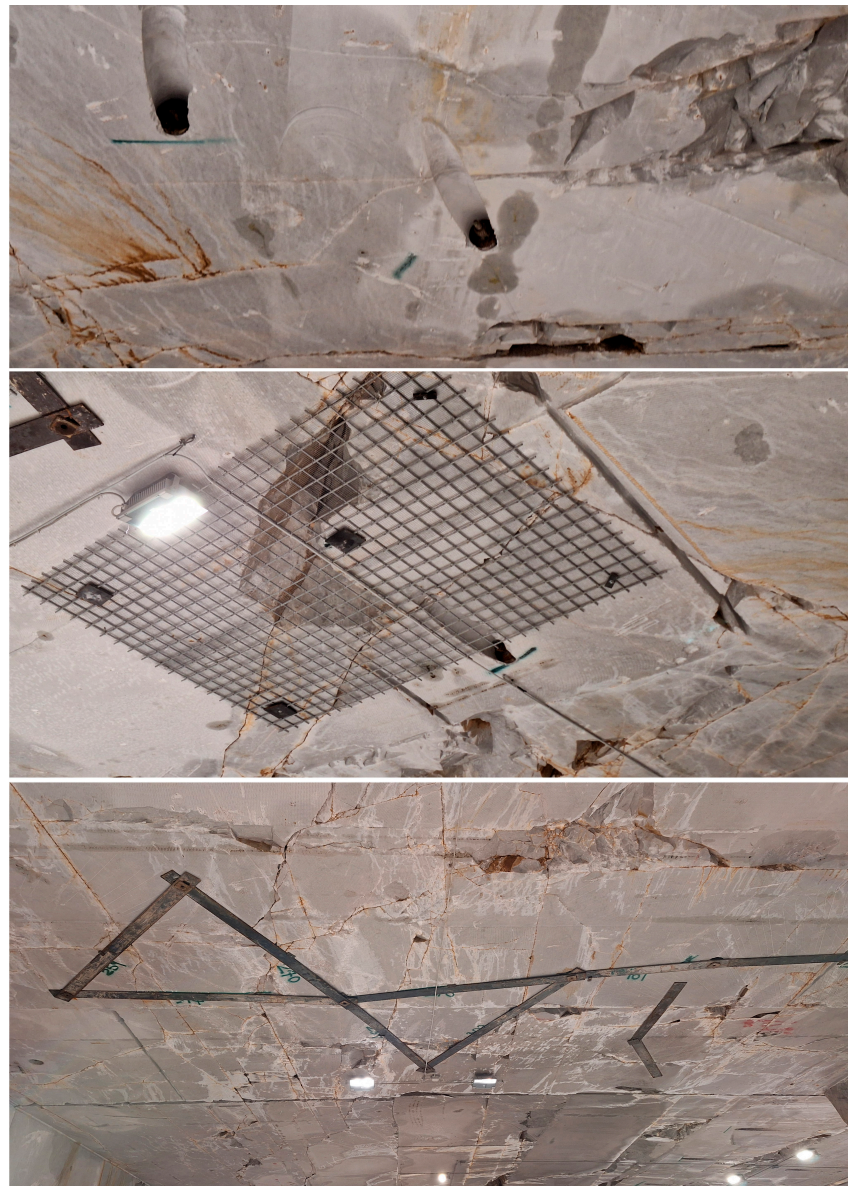
Figure 23. Examples of active supports installed in the roof of the underground tunnels.
