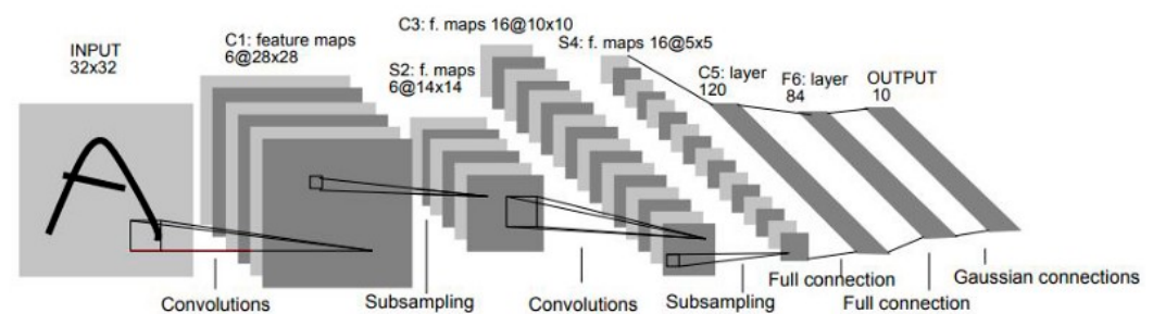
Figure 1. Architecture of LeNet-5 [12].
