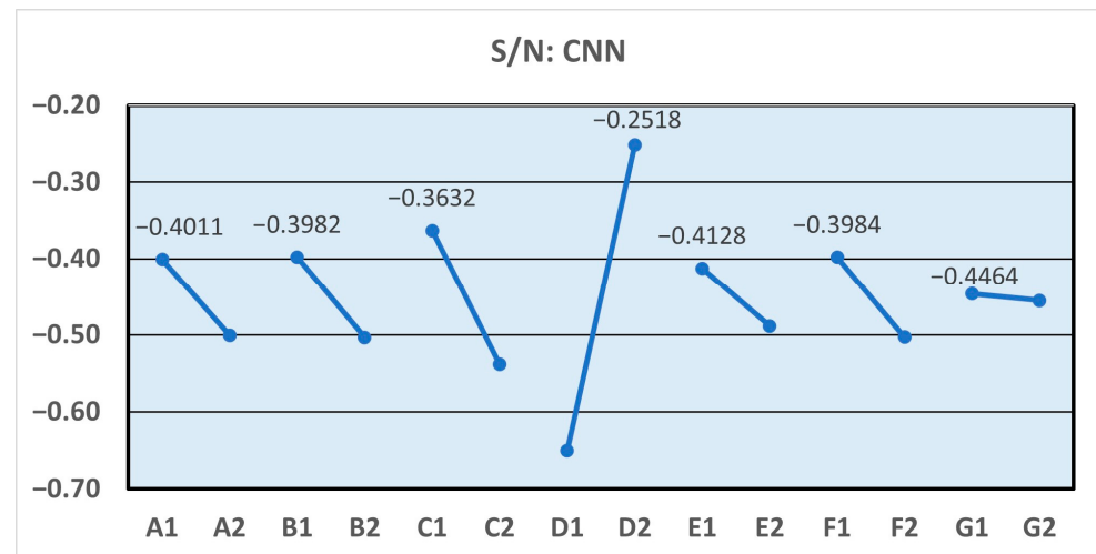
Figure 5. Factor S/N ratio response plot: Convolutional neural networks.
