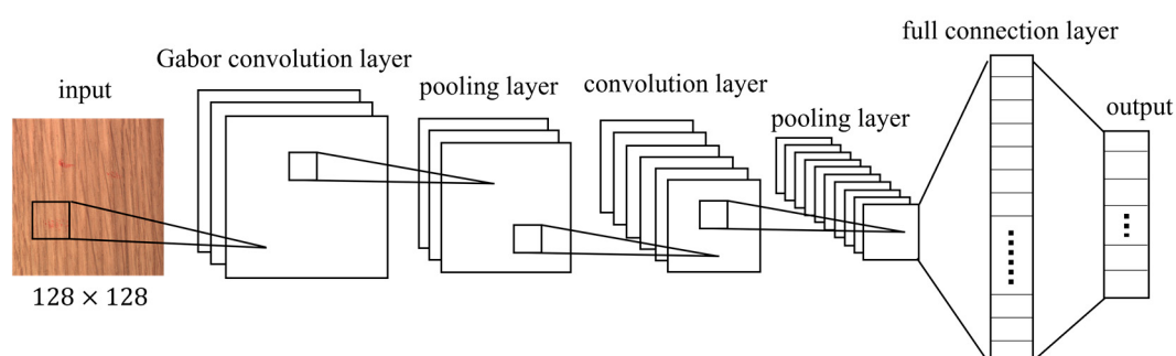
Figure 2. Architecture of Gabor convolutional networks.
