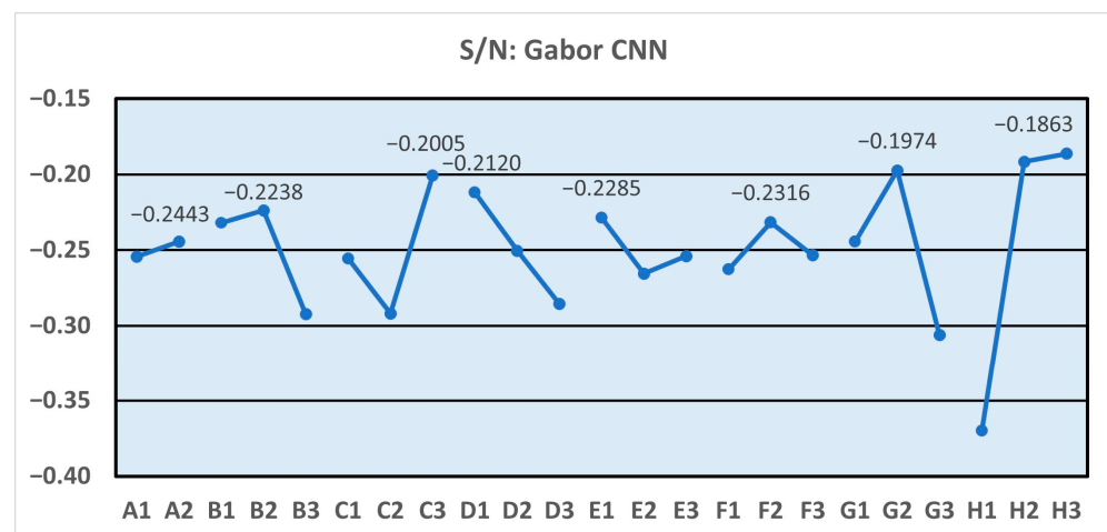
Figure 4. Factor S/N ratio response plot: Gabor convolutional networks.
