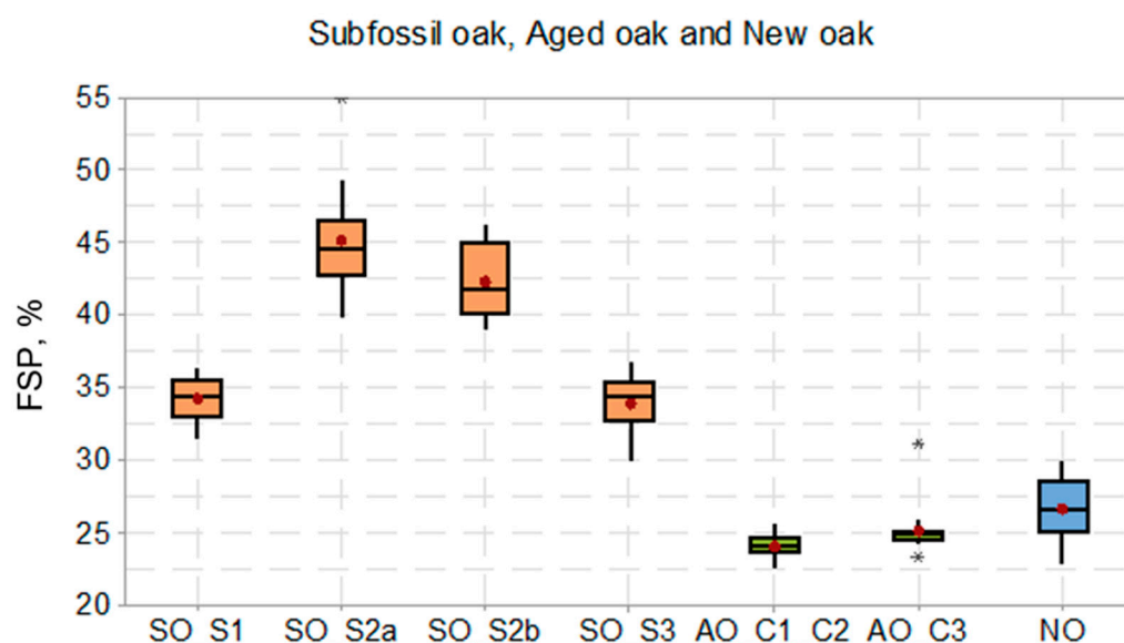
Figure 5. Box plots of FSP values, illustrating the variation in this property among the different assortments of oak wood and dispersion of data in each group. Note: Box plots include median value line, mean (average) value (brown point), whiskers for minimum and maximum values and outliers (*).
