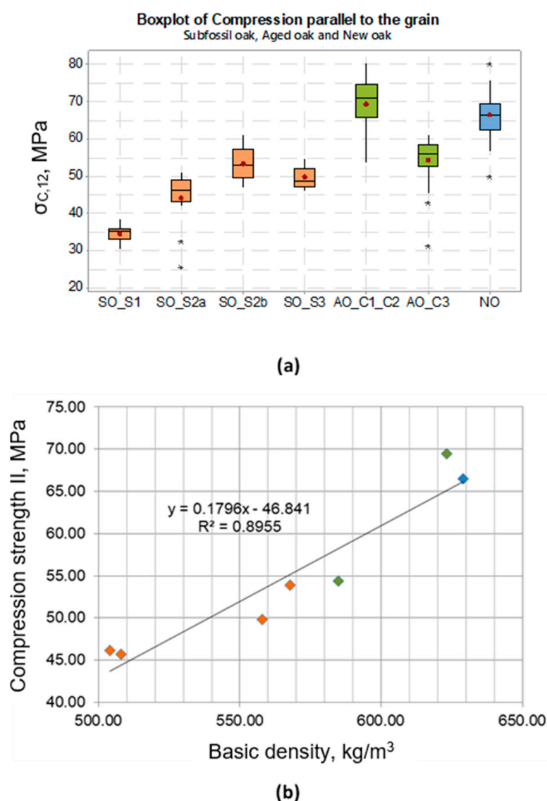
Figure 6. Ultimate compression stress parallel to grain: (a) Box plots illustrating variation among the different assortments of oak wood and dispersion of data in each group; (b) linear correlation with basic density. Note: Box plots include median value line, mean (average) value (red point),
