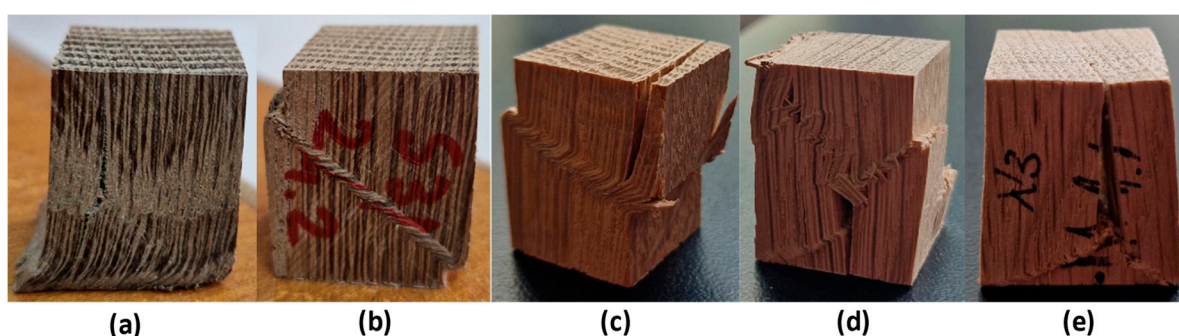
Figure 7. Exemplification of the main types of wood failure occurring by compression parallel to grain: (a) sliding of fibers; (b,c) break along one plane of minimum resistance, with a longitudinal crack (c); (d,e) break along two or more planes of minimum resistance with longitudinal cracks.
