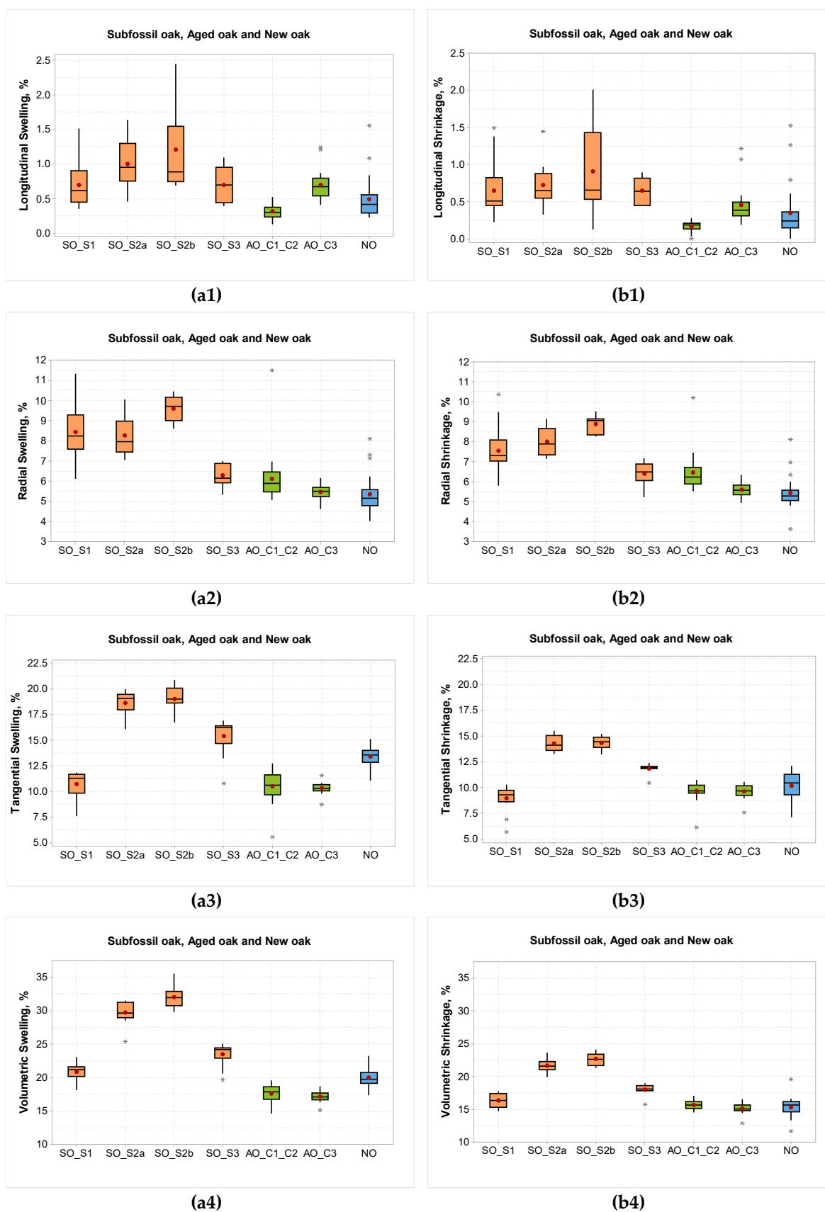
Figure 4. Box plots of total swelling (a1–a4) and total shrinkage coefficients (b1–b4), illustrating the variation in these values among the different assortments of oak wood and dispersion of data in each group. Note: Box plots include median value line, mean (average) value (red point), whiskers for minimum and maximum values and outliers (*).
