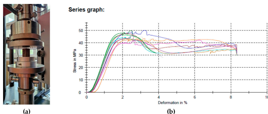
Figure 2. Determination of compression strength: (a) detail of ZwickRoell universal machine equipped with compression device; specimen positioned for testing; (b) examples of stress–deformation diagrams automatically registered (different colours represent different samples) .
