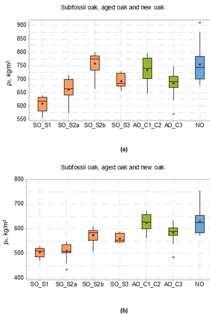
Figure 3. Box plots of oven-dried density (a) and basic density (b) illustrating the variation in these values among the different assortments of oak wood and dispersion of data in each group. Note: Box plots include median value line, mean (average) value (red dot), whiskers for minimum and maximum values and outliers (*).
