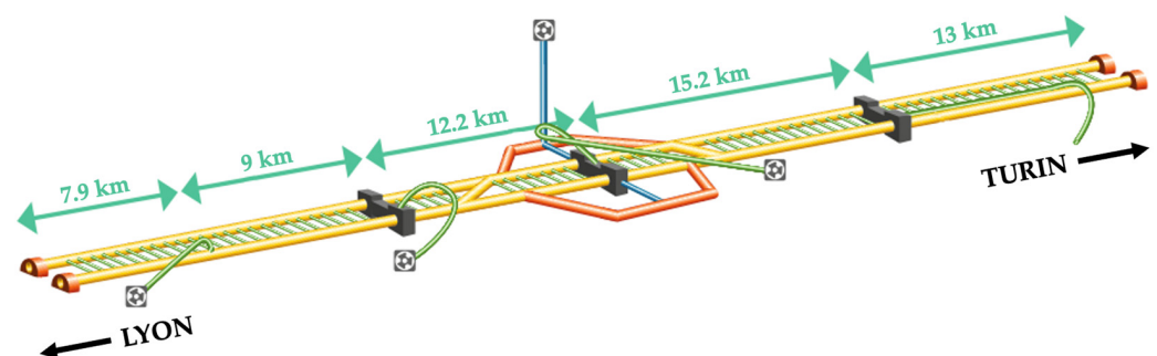
Figure 5. Summary view of the Mont Cenis Base Tunnel (modified from [33]).
