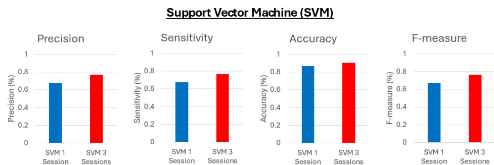
Figure 30. Comparing performance metrics for SVM classifiers utilizing data from one session and the complete dataset of three sessions of data.
