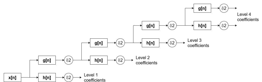
Figure 17. Discrete Wavelet Transform decomposition, block diagram form, with 4 levels of decomposition.
