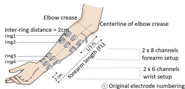
Figure 3. GRABMyo dataset setup for electrodes on the forearm [12].
