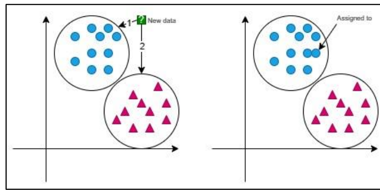
Figure 21. Visualization of K-Nearest Neighbor classes and classification method.
