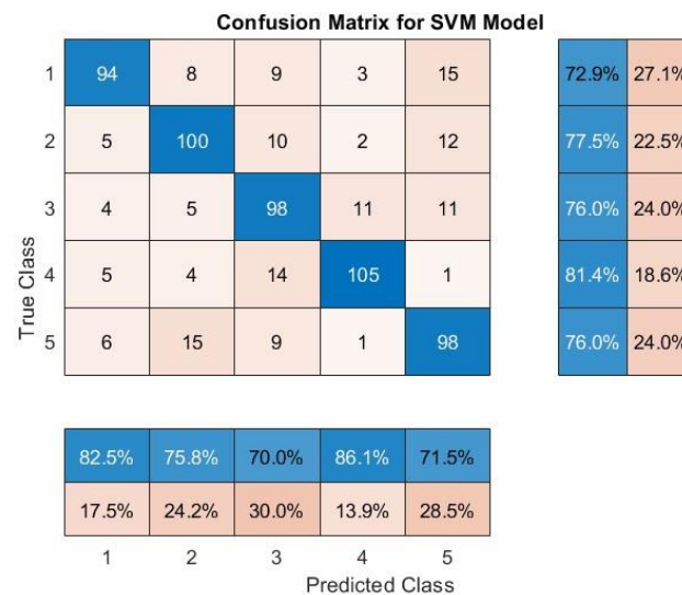
Figure 28. Confusion matrix for the SVM model using data from the complete dataset of three sessions of data.
