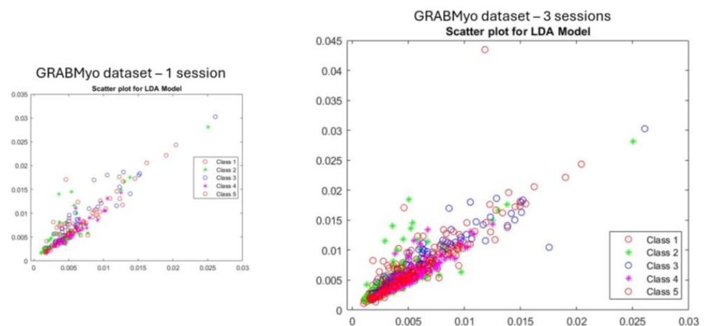
Figure 27. Comparison of scatter plots between one session and the complete dataset of three sessions of data.
