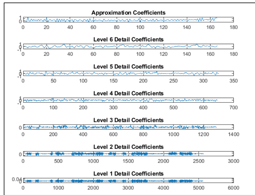
Figure 18. Discrete Wavelet Transform decomposition with 6 levels of decomposition.
