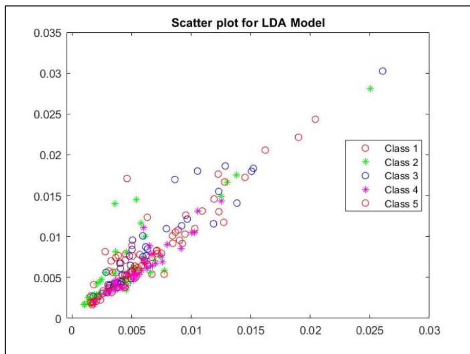
Figure 25. Scatter plot illustrating the classification of 215 EMG samples using the LDA–SVM model.
