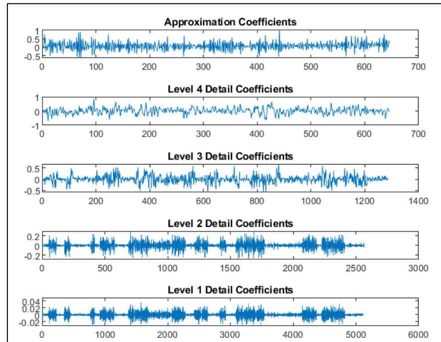
Figure 19. Discrete Wavelet Transform decomposition, analysis form, with 4 levels of decomposition.
