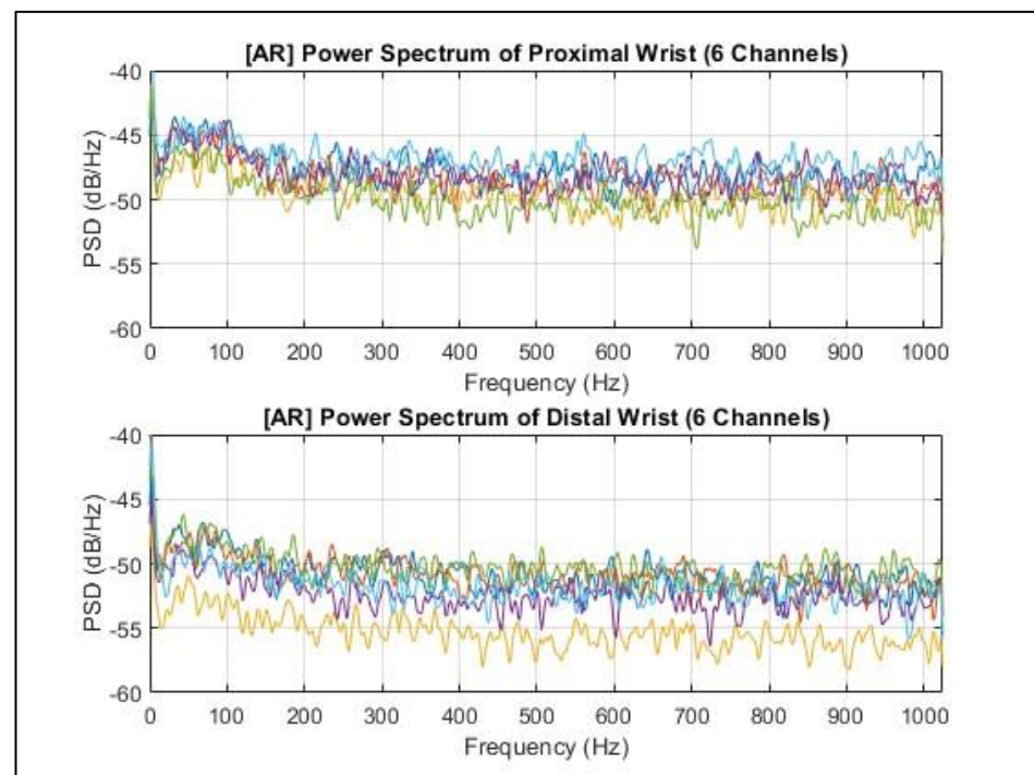
Figure 12. PSD analysis of EMG signals captured from the forearm after average referencing.
