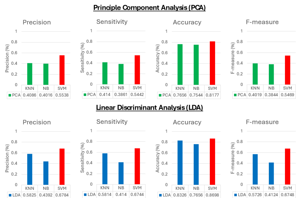
Figure 29. Performance metrics for KNN, NB, and SVM classifiers using data from one session.
