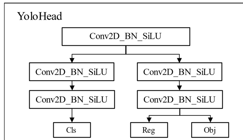
Figure 2. Yolo Head Structure Diagram.
