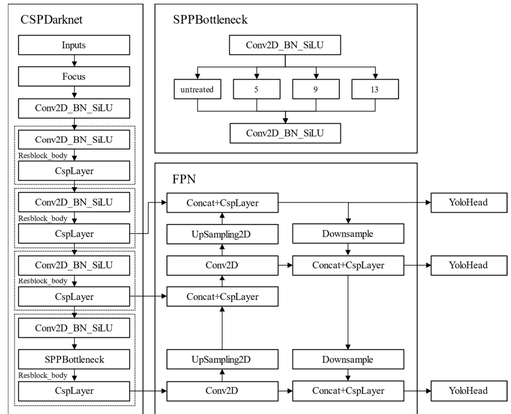
Figure 1. YoloX-tiny Network Structure.
