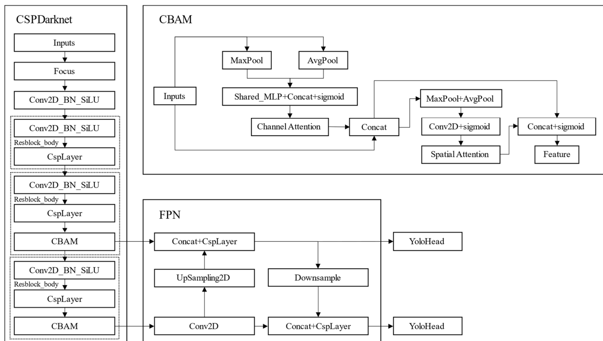
Figure 3. Improved Yoloxy-tiny Network Structure.
