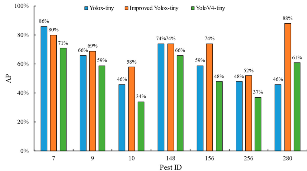
Figure 10. Comparative Results of Pest Detection by Category.
