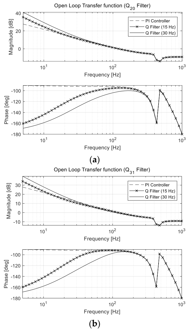
Figure 8. Open-loop transfer function of DOB-based anti-shock controller for FSM control systems: (a) Q_{20} and (b) Q_{31} filters.
