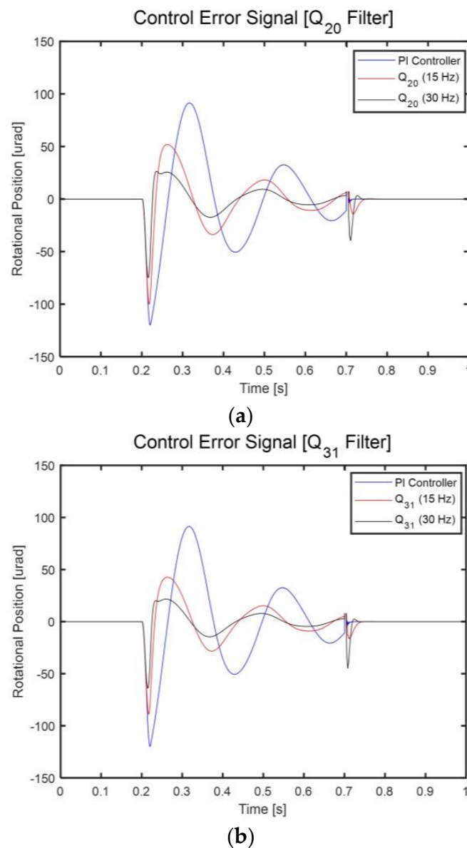
Figure 10. Simulated performance results obtained using DOB-based anti-shock controller for FSM control systems: (a) Q_{20} filter (15/30 Hz), and (b) Q_{31} filter (15/30 Hz).
