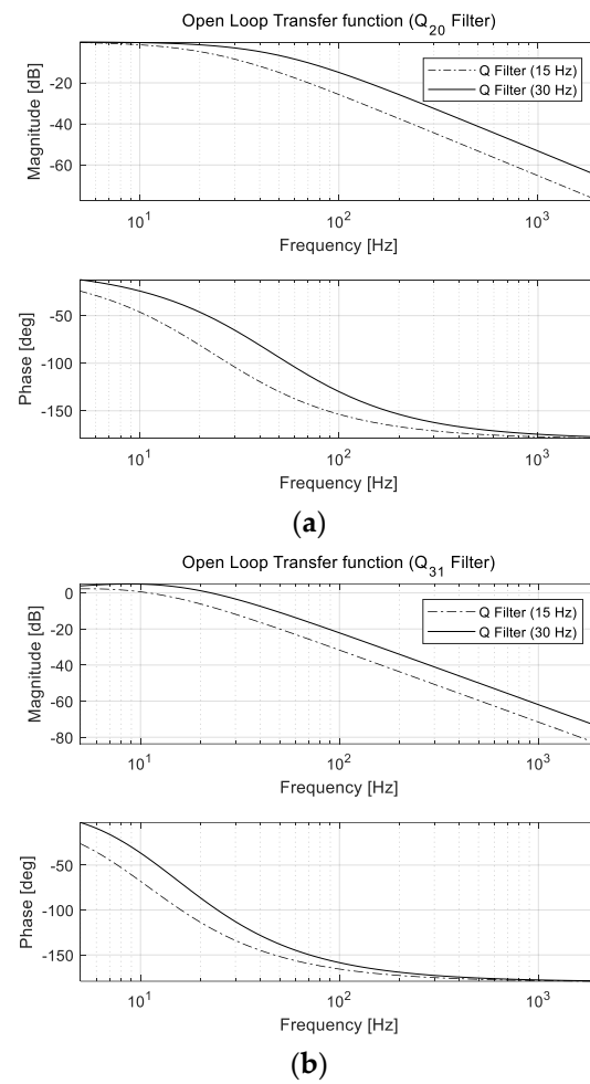
Figure 7. Open-loop transfer function of Q filters used in DOB-based anti-shock controller for FSM control systems: (a) Q_{20} and (b) Q_{31} filters.
