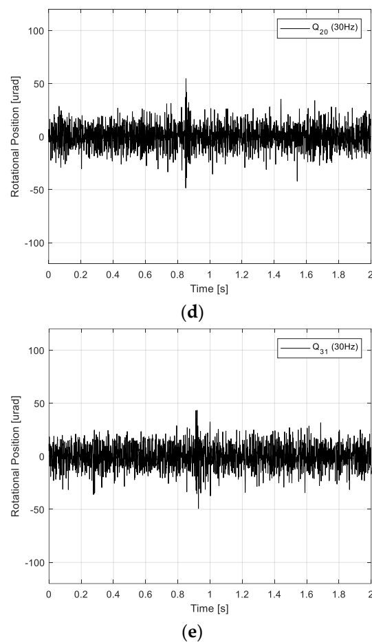
Figure 11. Performance results obtained using DOB-based anti-shock controller for FSM control systems: (a) PI controller, (b) Q_{20} filter (15 Hz), (c) Q_{31} filter (15 Hz), (d) Q_{20} filter (30 Hz), and (e) Q_{31} filter (30 Hz).
