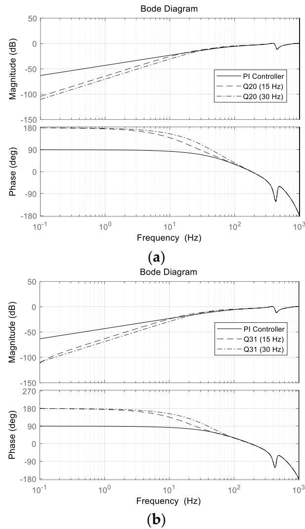
Figure 9. Disturbance-rejection performance of DOB-based anti-shock controller for FSM control systems: (a) Q_{20} and (b) Q_{31} filters.
