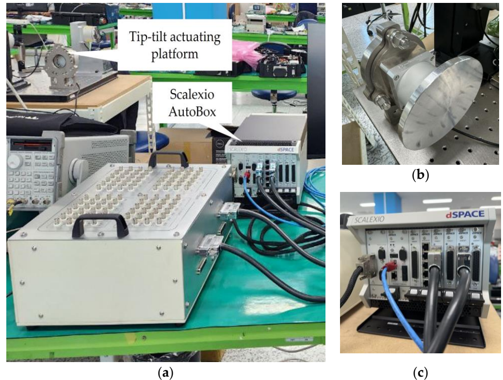
Figure 2. (a) FSM control system; (b) tip-tilt actuating platform (PI Ceramic GmbH); and (c) Scalexio AutoBox (dSPACE).
