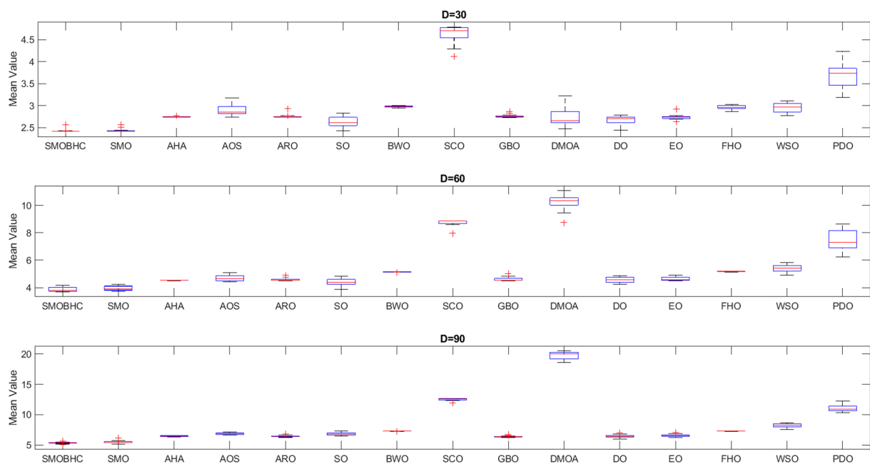
Figure 21. Boxplot graphs of mean values relative to all algorithms for battlefield 3 with D = 30, 60 , and 90 .
