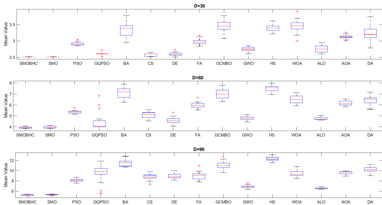
Figure 16. Boxplot graphs of mean values relative to all algorithms for battlefield 2 with D = 30, 60 , and 90 .
