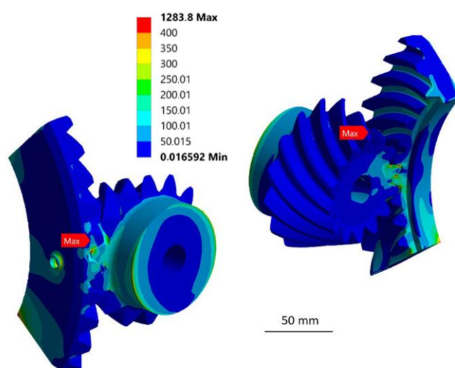
Figure 19. Distribution of equivalent von Mises stresses on ring gear.
