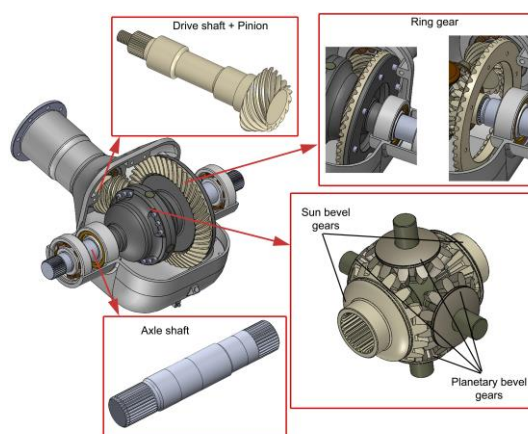
Figure 4. CAD model of ODT with bevel gears.
