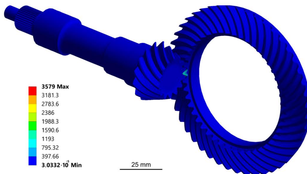
Figure 8. Equivalent stress fields according to von Mises in MPa, pinion and bevel gear.
