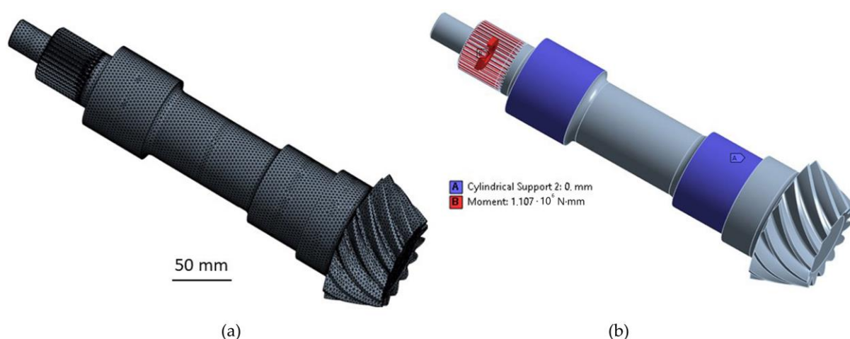
Figure 11. Drive shaft finite element model: (a) finite element mesh; (b) boundary conditions.
