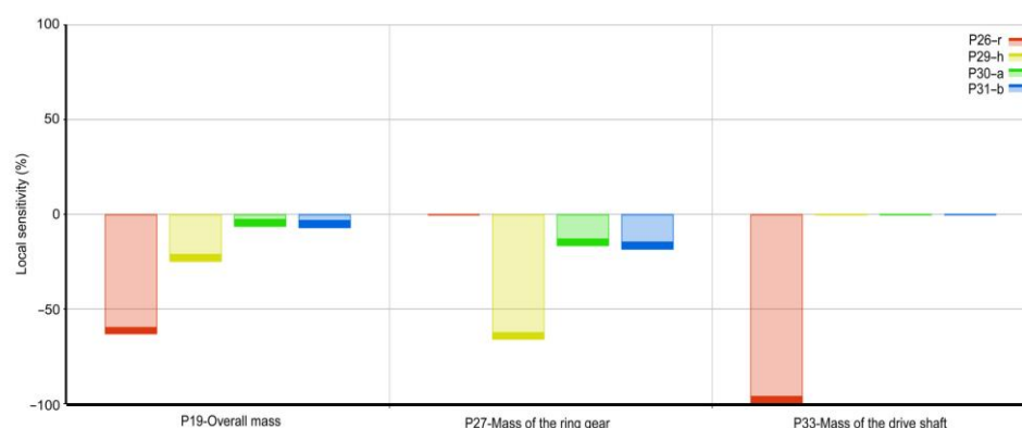
Figure 17. Sensitivity indices for the responses: overall mass, mass of the ring gear and mass of the drive shaft.
