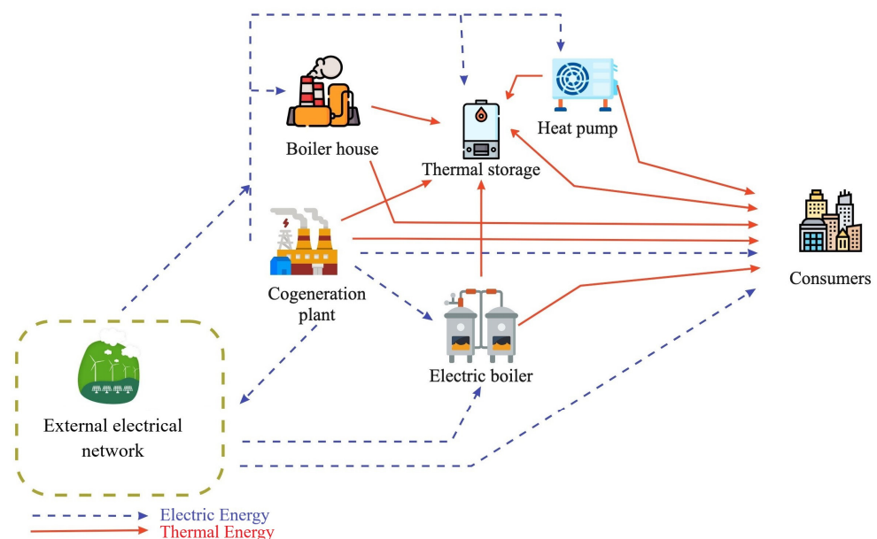
Figure 7. Scheme of a DHS with various sources of thermal energy.
