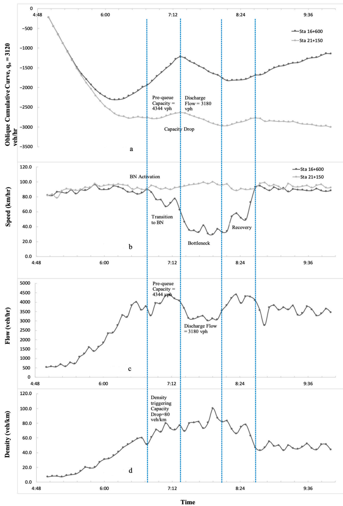
Figure 2. Oblique cumulative curves, speed, flow, and density on 1 June 2022.
