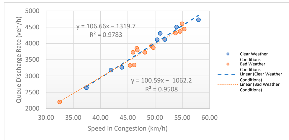
Figure 4. Relationship between queue discharge rate and speed in congestion (clear and bad weather conditions separated).
