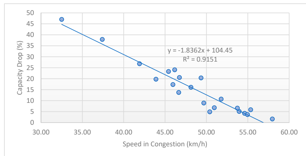
Figure 5. Relationship between the capacity drop and speed in congestion.
