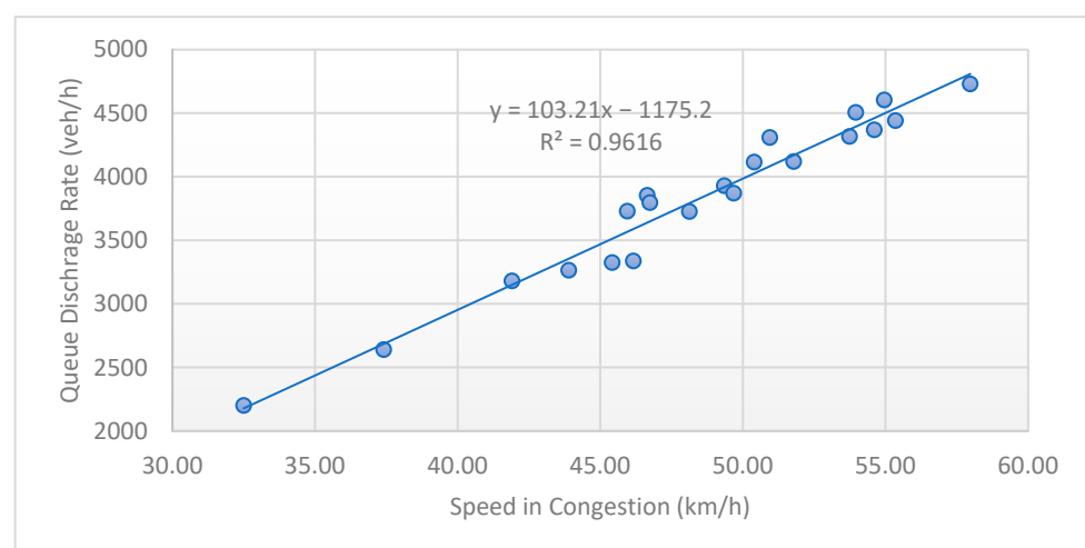
Figure 3. Relationship between queue discharge rate and speed in congestion (all data points).
