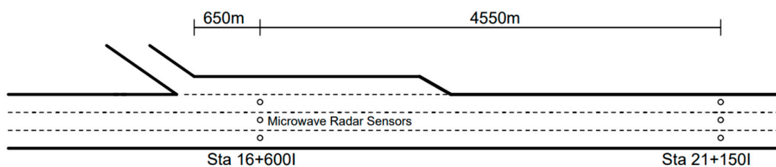
Figure 1. On-ramp bottleneck data site, Burapha Withi Expressway, Bangkok, Thailand.
