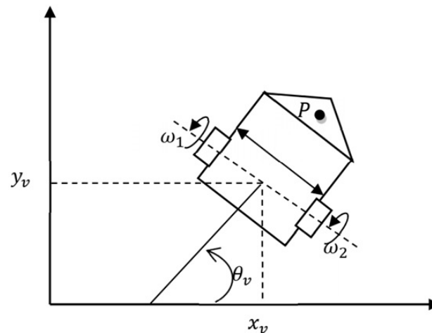
Figure 4. Considered car-type vehicle (target).
