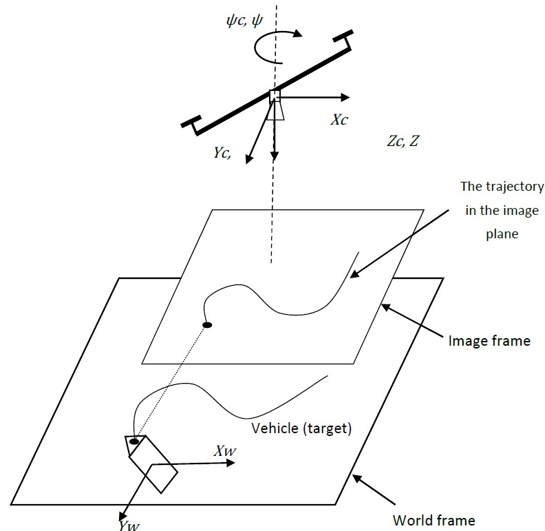
Figure 2. Quadrotor coordinate system vs. Cartesian world coordinate system.
