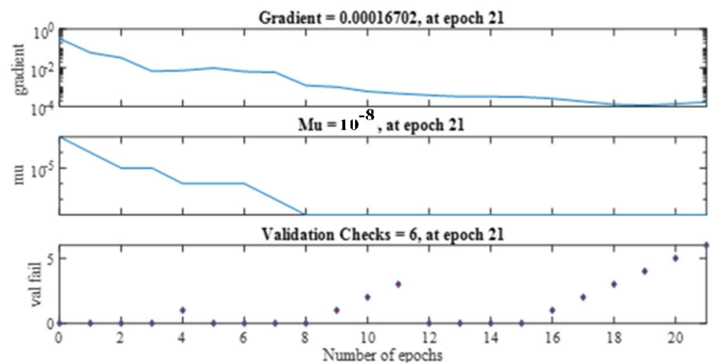
Figure 7. Training state of ANN for 4-10-1.
