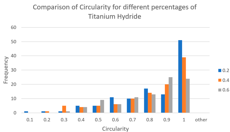
Figure 11. Comparison of distribution of circularity for different amount of \text{TiH}_2 .
