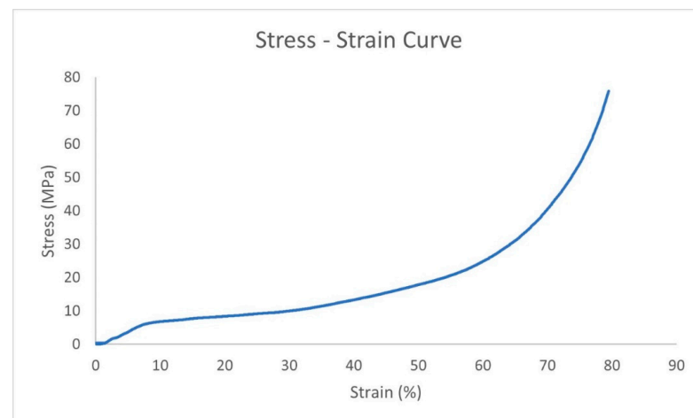
Figure 3. Stress–strain curve for sample 1 (0.2% TiH 2 , 2.8% SiC).
