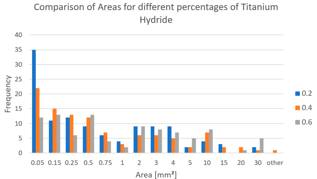
Figure 9. Comparison of distribution of area for different compositions of \text{TiH}_2 .
