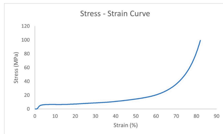
Figure 6. Stress–strain curve for sample 4 (0.2% TiH 2 , 6% SiC).
