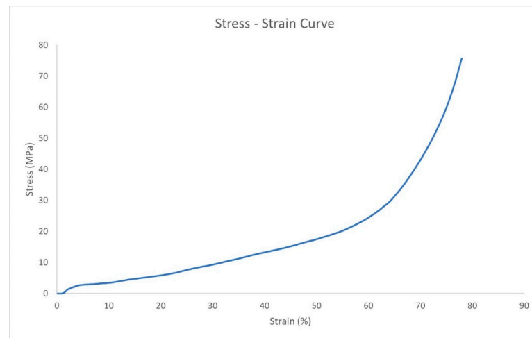
Figure 4. Stress–strain curve for sample 2 (0.4% TiH 2 , 2.8% SiC).
