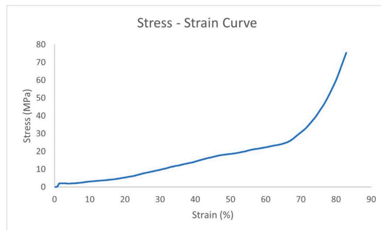
Figure 5. Stress–strain curve for sample 3 (0.6% TiH 2 , 2.8% SiC).
