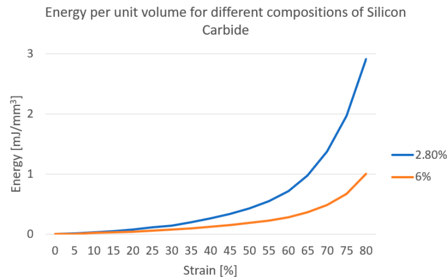
Figure 8. Energy per unit volume for different compositions of \text{SiC} .
