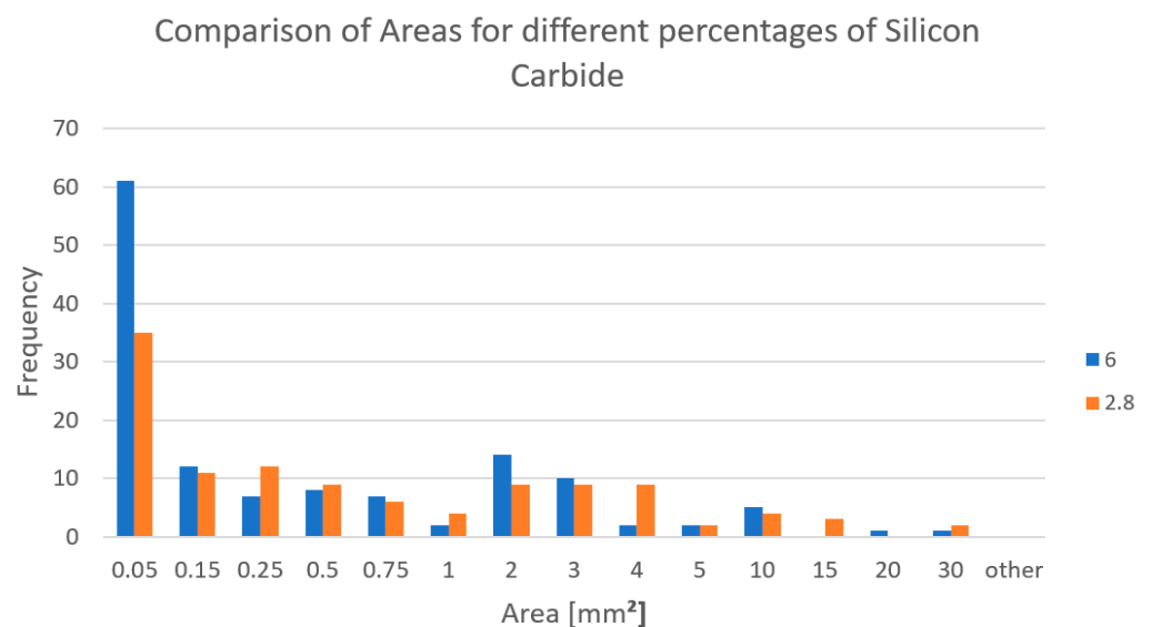
Figure 10. Comparison of distribution of area for different amount of \text{SiC} .
