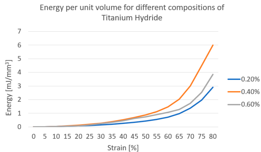
Figure 7. Energy per unit volume for different compositions of \text{TiH}_2 .
