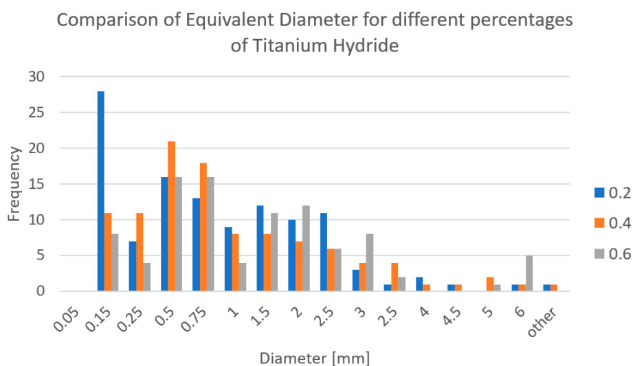
Figure 13. Comparison of distribution of equivalent diameter for different amount of \text{TiH}_2 .
