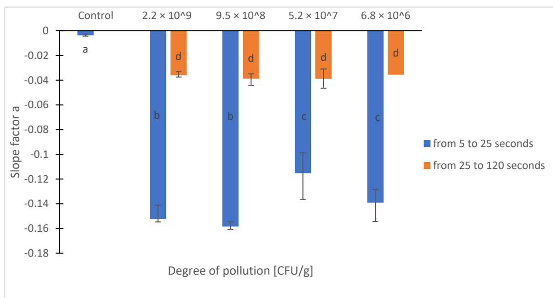
Figure 3. Comparison of temperature regression coefficients (mean values and standard deviation) relative to the time after the activation of B. subtilis bacteria contamination samples: 2.2 \times 10^9 CFU/g, 9.5 \times 10^8 CFU/g, 5.2 \times 10^7 CFU/g, and 6.8 \times 10^6 CFU/g; a–d—different letters on the bars indicate statistically significant differences between the samples by Tukey's test ( p < 0.05 ).
