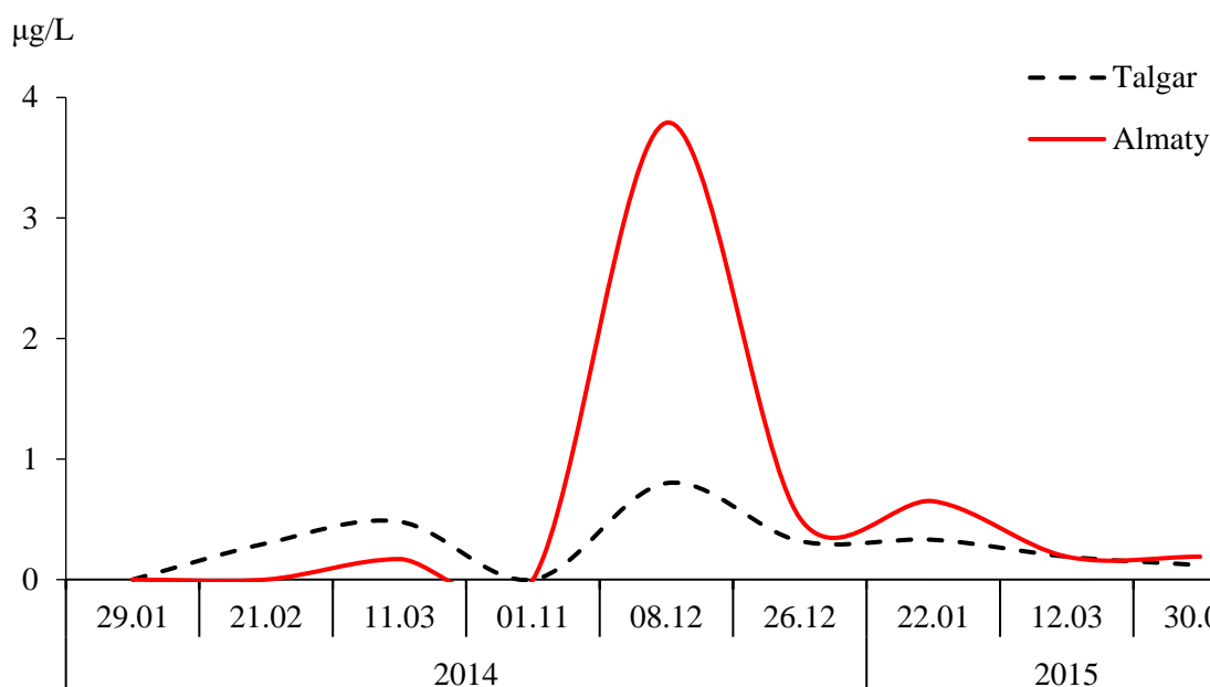
Figure 2. PCB content changes in the snow samples at the observation points of Almaty and Talgar cities.
