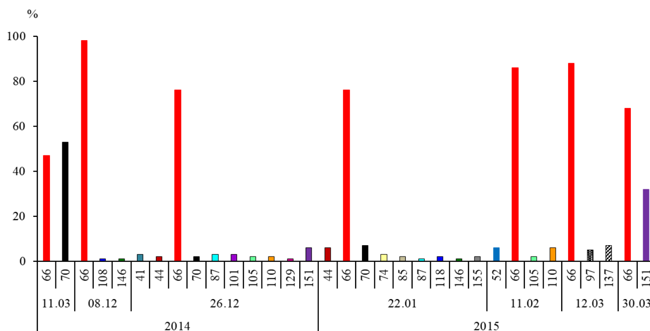
Figure 4. Relative content of PCB congeners in solid precipitations in the territory of Almaty city.
