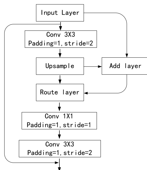
Figure 4. The VaryBlock module is designed according to the residual mechanism and feature fusion method of add and concatenate.
