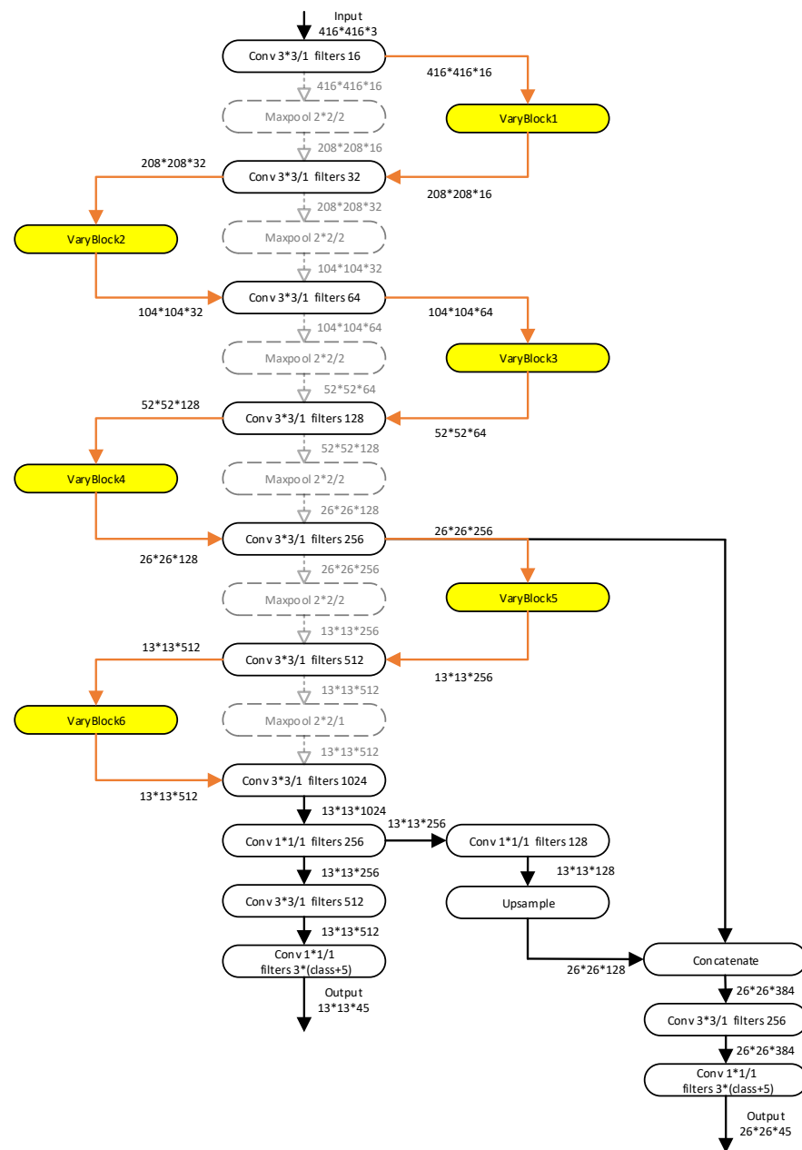
Figure 2. Network structure of the improved YOLO-Tiny(v3) object detection. The color part is the added module, the gray part is the replaced structure, and the rest is the reserved structure.
