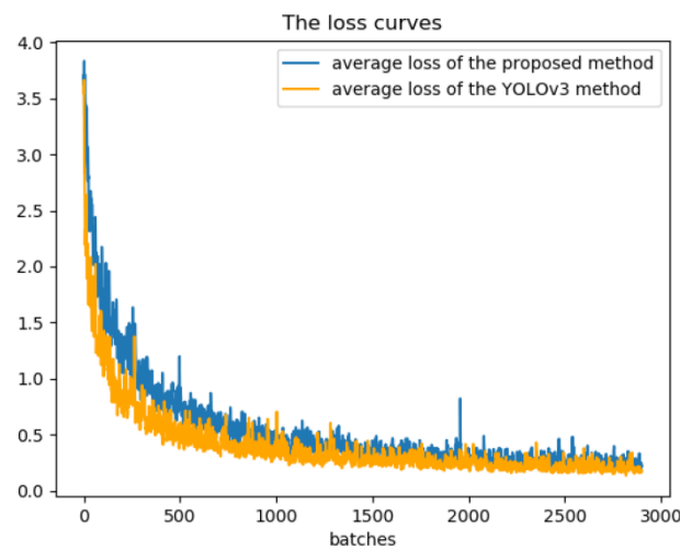
Figure 9. The training loss curves of our proposed method and YOLOv3-Tiny.
