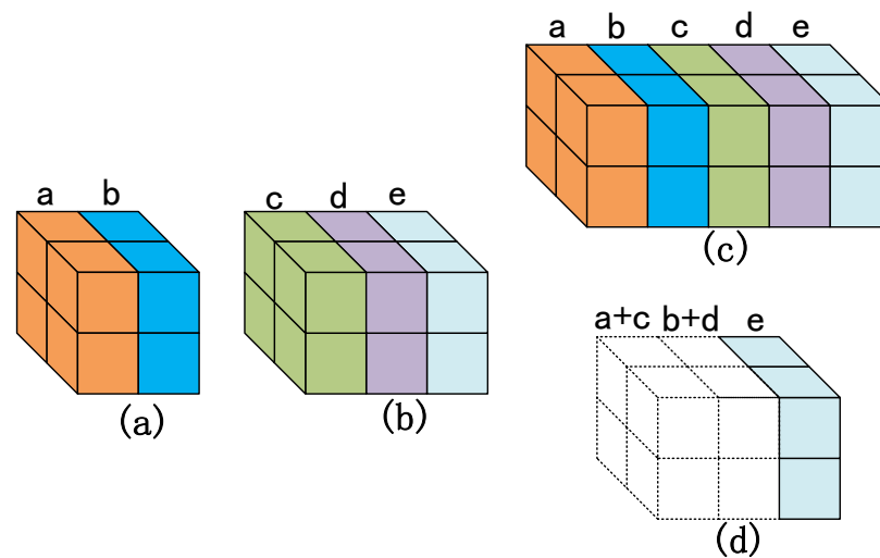
Figure 3. Operation of Add layer and Route layer; (a) A = [a, b] ; (b) B = [c, d, e] ; (c) C = [a, b, c, d, e] ; (d) D = [a+c, b+d, e] ; a, b, c, d are all feature maps; C is Route layer and D is Add layer.
