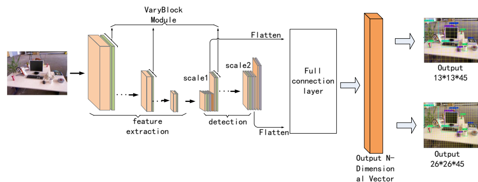
Figure 1. Improved YOLOv3-Tiny object detection algorithm framework.
