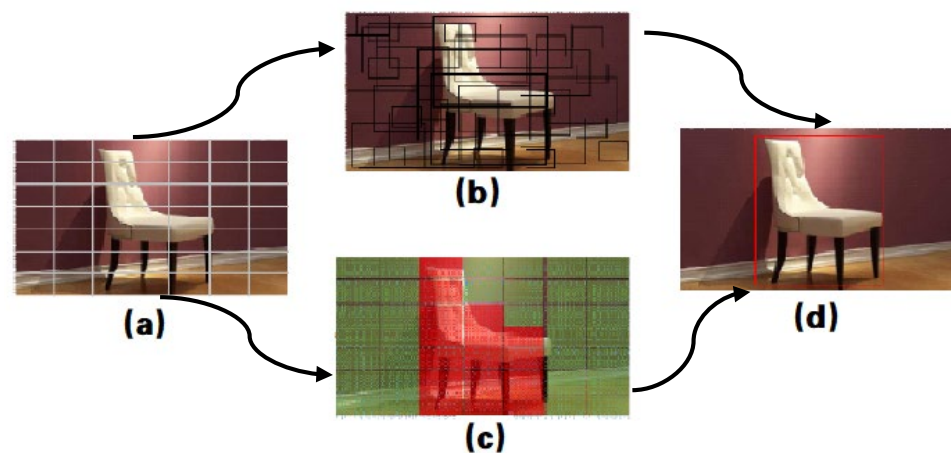
Figure 6. The prediction process of the improved YOLOv3 object detection; The input image is divided into an equal-sized s \times s grids (a); each grid includes three different scales and each scale owns three bounding boxes with different sizes (b,c) to predict the object (d).
