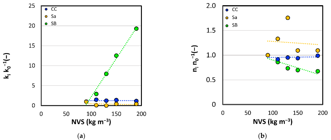
Figure 1. (a) Variation of consistency coefficient of conditioned TBS with respect to unconditioned sludge k_i k_0^{-1} as a function of NVS concentration. (b) Variation of flow behaviour index of conditioned TBS with respect to unconditioned sludge n_i n_0^{-1} as a function of NVS concentration. Dot lines represents the linear tendency. CC: calcium carbonate; Sa: sand; SB: sodium bentonite.
