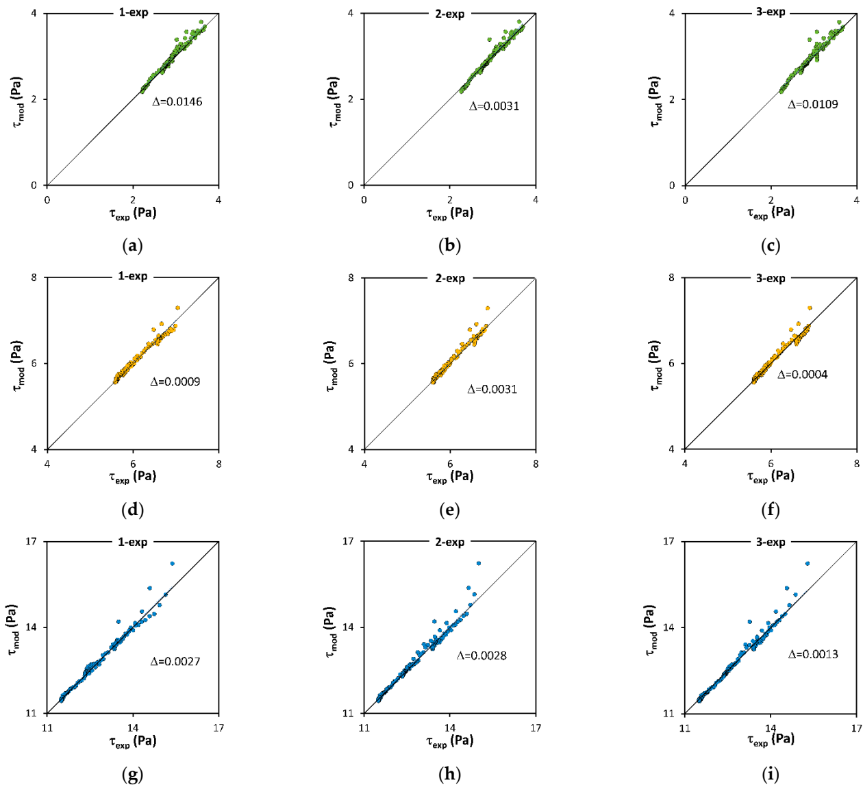
Figure 3. Comparison between experimental data and single, double, and triple-exponential models to describe the shear stress as a function of time. (a–c) are referred to 100 s -1 . (d–f) are referred to 400 s -1 . (g–i) are referred to 1000 s -1 .
