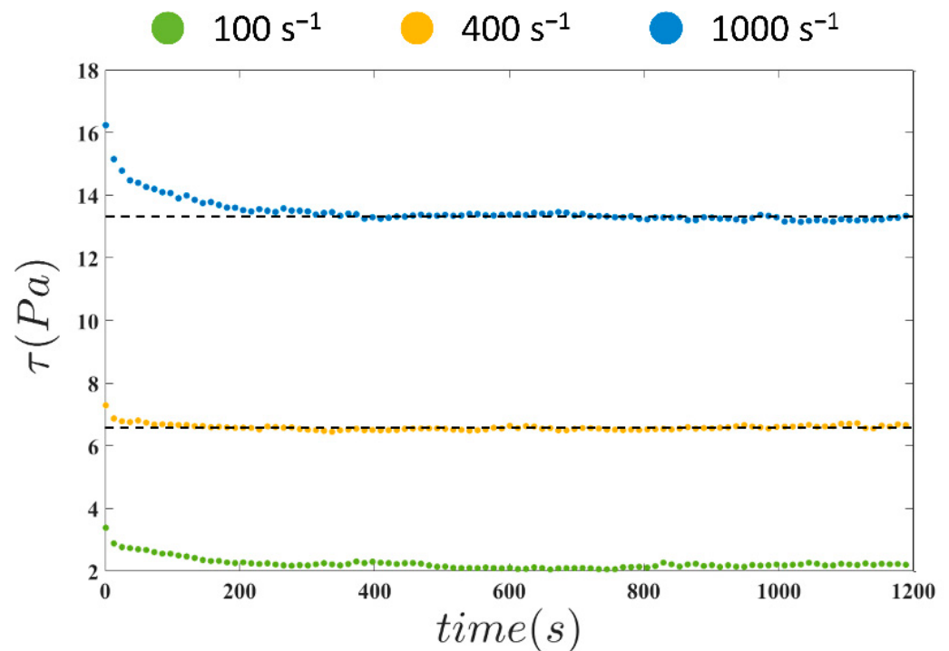
Figure 2. Shear stress as a function of time for different values of applied shear rate.
