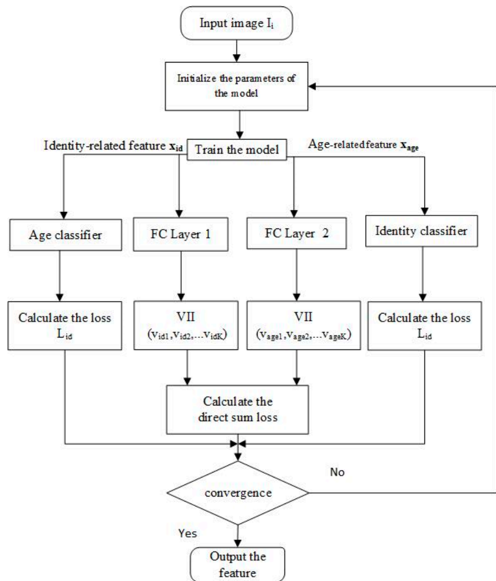
Figure 5. The flow chart of the training process. The whole loss is obtained through the identity classifier, age classifier, and direct sum modules.
