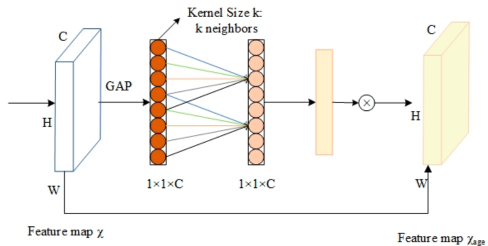
Figure 3. Diagram of the ECA block.
