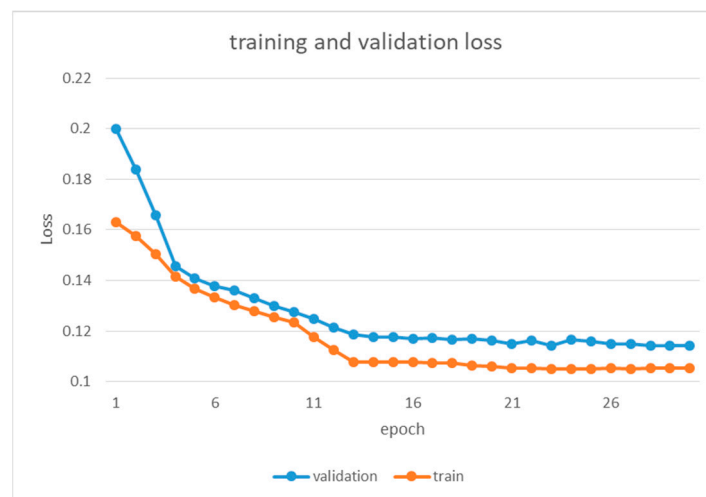
Figure 8. Trend of training and validation loss.
