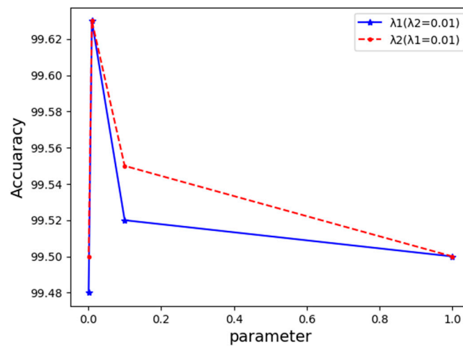
Figure 9. Face verification accuracy on the CACD-VS dataset with various values for \lambda_1 and \lambda_2 .
