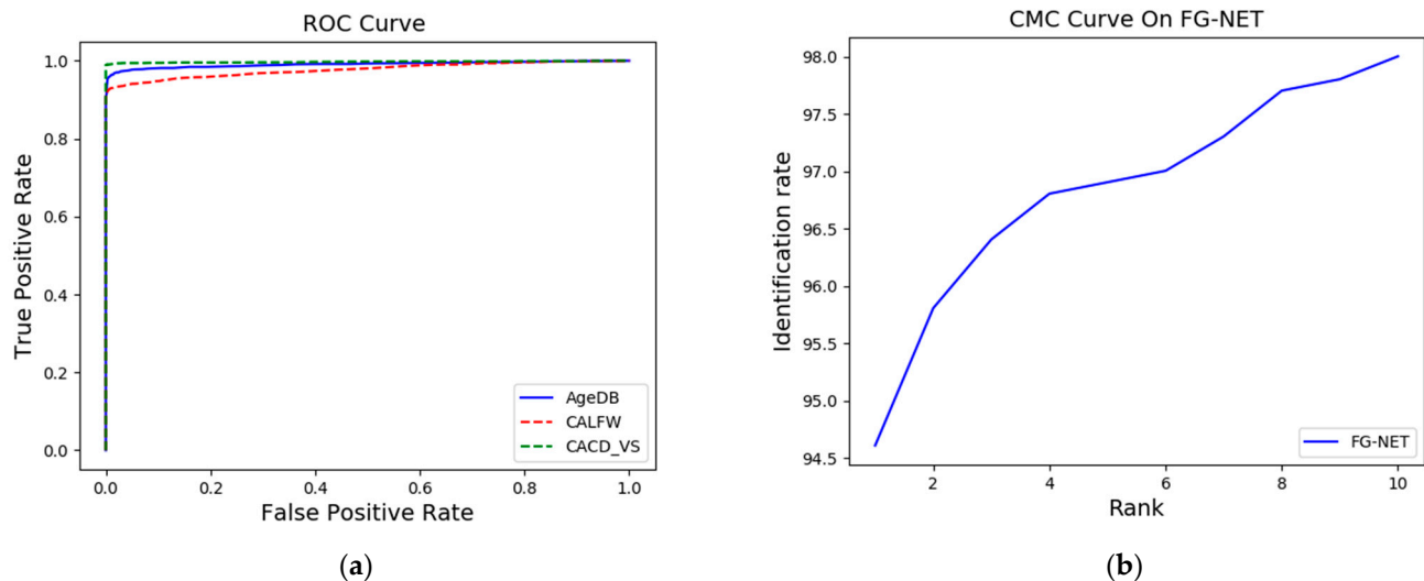
Figure 10. Face recognition performance of our model (a) ROC curves on CACD-VS, CALFW, AgeDB-30. (b) CMC curve on FG-NET.
