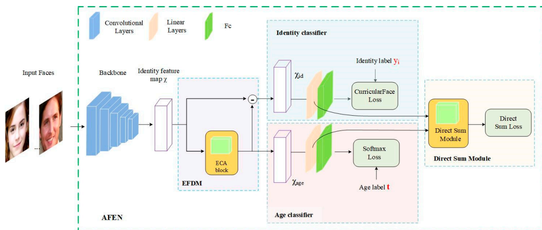
Figure 2. Overall framework of the proposed AFEN and its training process.
