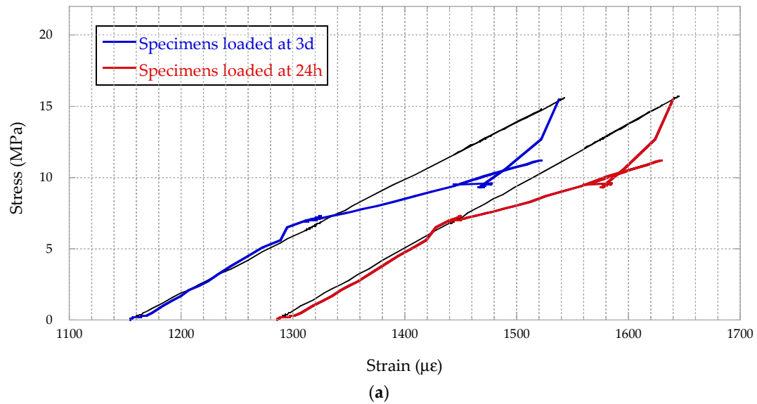
Figure 11. Evolution of the modulus of elasticity of FRC with age.
