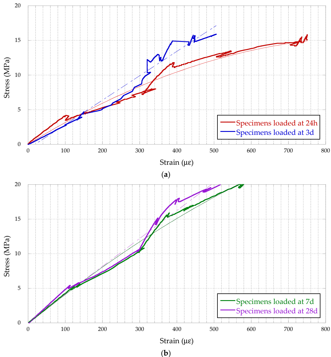
Figure 10. Tension-deformation curve during loading of the specimens: (a) FRC specimens loaded at 15 MPa; (b) FRC specimens loaded at 20 MPa.
