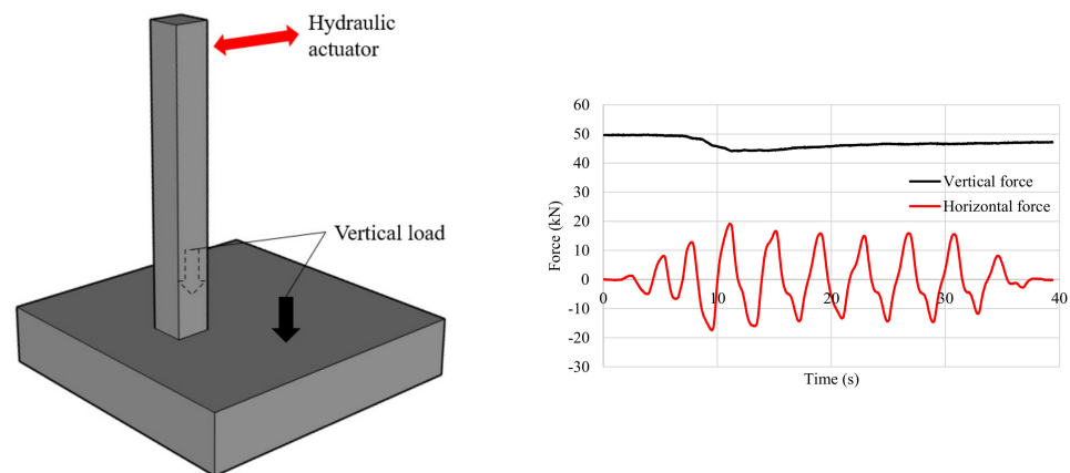
Figure 2. Load application Phase II—low density sand (m).
