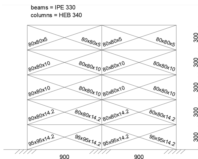
Figure 10. Braced frame.
