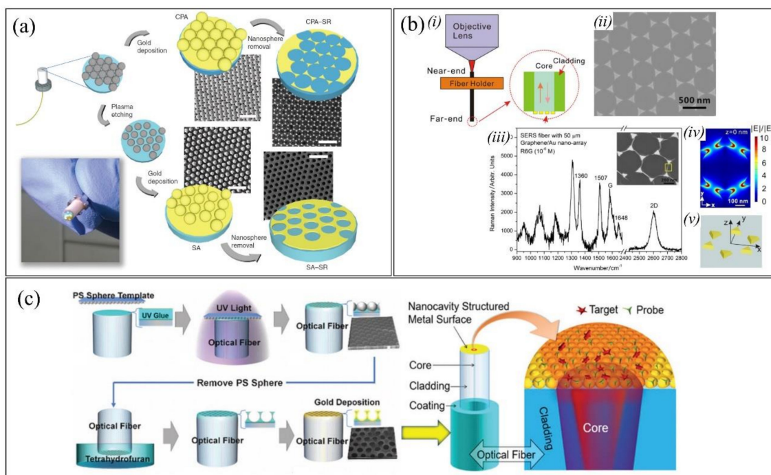
Figure 2. (a) Fabrication procedure for creating four different fiber tip nanoprobe structures and SEM images (scale bar = 3 \mu\text{m} ) of real samples obtained using 1- \mu\text{m} nanospheres, and photograph of a fiber tip showing an iridescent nanopattern. Reproduced from Ref. [52]. (b) Fiber probe with hybrid graphene/Au nano-triangle nanostructuration: schematic diagram of the experiment setup (i), SEM image of Au nano-triangle array (ii), R6G Raman spectrum obtained by fiber probe (iii), electric field magnitude mapping along x-y plan for z = 0 \text{ nm} (iv) and schematic model of Au triangle array (v). Reproduced from Ref. [57] with permission from 2017 WILEY-VCH Verlag GmbH and Co. KGaA, Weinheim, Germany. (c) Fabrication procedure for the nanocavities-patterned fiber probe obtained by combining colloidal assembly and UV nanoimprinting, which includes the coating, patterning, and metallization of the cavities on the fiber end face. Reproduced from Ref. [59] with permission from 2019 WILEY-VCH Verlag GmbH and Co. KGaA, Weinheim, Germany.
