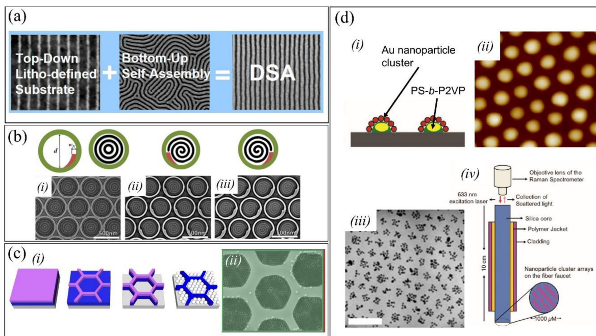
Figure 4. (a) Representation of the directed self-assembly (DSA) approach: the combination of block-copolymer self-assembled into organized nanoscale structures with lithographically defined structures acting as guiding patterns, produces highly regular patterns of lines/spaces. Reproduced from Ref. [79] (b) Schematic (top) and experimental (bottom) examples of concentric rings (i) and spirals of right-handed (ii) or left-handed (iii) chirality, formed by a block copolymer self-assembled in circular (i) and notched (ii,iii) templates. The template diameters in (i–iii) are 350 nm. Reproduced from Ref. [80] with permission from 2017 IOP Publishing Ltd. (c) Schematic representation of the lithographic process to obtain a hexagonal pattern for DSA of colloidal particles (i) and SEM micrograph of the assembled particles in the hexagonal pattern. Reproduced from Ref. [82]. (d) Schematic representation of gold nanoparticle clusters grown around PS- b -P2VP inverse micelles assembled on a substrate (i); AFM image of the array of PS- b -P2VP micelles (ii); SEM micrograph of the array of Au nanoclusters resulting from the decoration of the BCP micelles (iii); schematic representation of the SERS analysis setup including the patterned optical fiber probe (iv). Reproduced from Ref. [83] with permission from the 2012 American Chemical Society.
