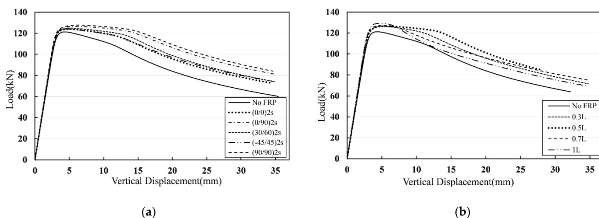
Figure 9. The effect of (a) ply distributions, and (b) retrofitted brace length, on the axial load-displacement curve of the retrofitted T2 joint.
