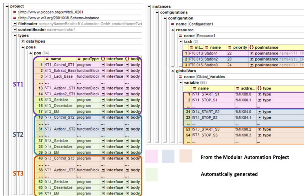
Figure 12. Example of a Flexible Automation Project containing the POU, data types, global variables and tasks associated to three Production Services (ST1–ST3).
