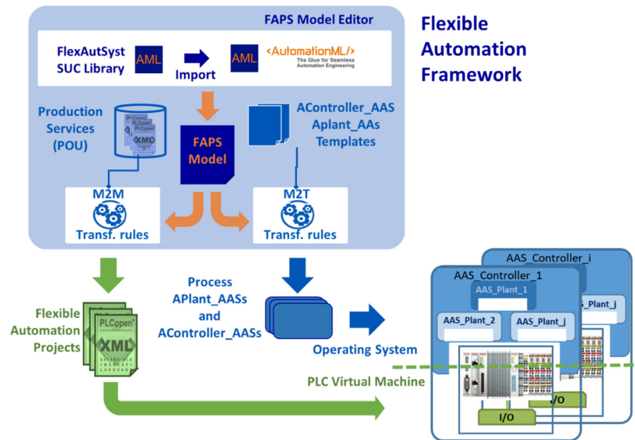
Figure 6. General Scenario of Flexible Automation Framework.
