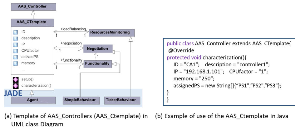
Figure 15. (a) Template of an AAS_Controller (AAS_CTemplate) in UML Class Diagram with detail of its methods and the states defined in its FSM and (b) Example of the use of the AAS_CTemplate in Java. The characterization method of the AAS_Controller element allows the customization of the parameters ID, description, IP, CPUfactor, memory and assignedPS for different AAS_Controller instances.
