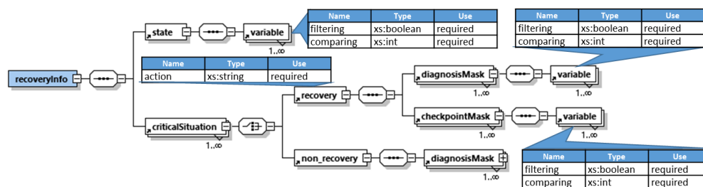
Figure 14. General Structure of the Diagnosis.xml file: Recovery information comprises the set of state variables to be analyzed as well as the set of critical situation masks. These masks allow to diagnose either recovery or non-recovery situations under controller failures/workloads balancing. This is performed by filtering a concrete set of state variables related to the condition to be diagnosed. This graphic was generated using Altova XMLSpy Version 2020.sp1.
