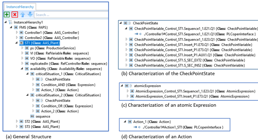
Figure 8. Flexible Automation control system design example with AutomationML Editor: (a) General Structure composed by three stations (ST1...ST3) controlled by two Controllers; (b) Characterization of the CheckPointState of the first critical situation identified in ST1; (c) Characterization of an atomic Expression: \text{Control\_ST1.Sequence1\_1.E23.Q1} = 1 AND \text{Control\_ST1.Insert\_P1.E73.Q1} = 1 ; and (d) Characterization of an Action.
