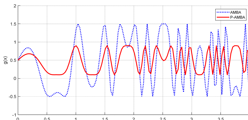
Figure 3. Generating function plotted with default values ( a = 0 , b = 0.5 , c = 0.8 , d = 0.5 , e = 0.4 , and g = 0.2 ).
