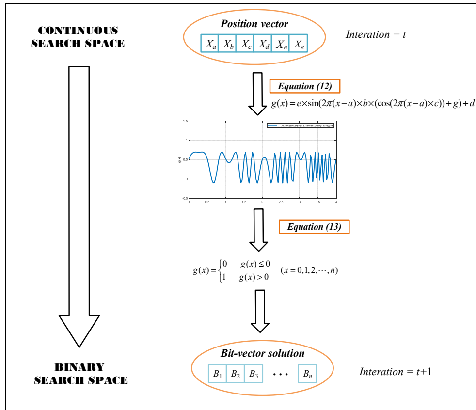
Figure 4. The process of mapping continuous search space to discrete search space.
