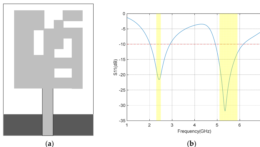
Figure 10. Final geometry (a) and S 11 curve (b) of the final antenna.
