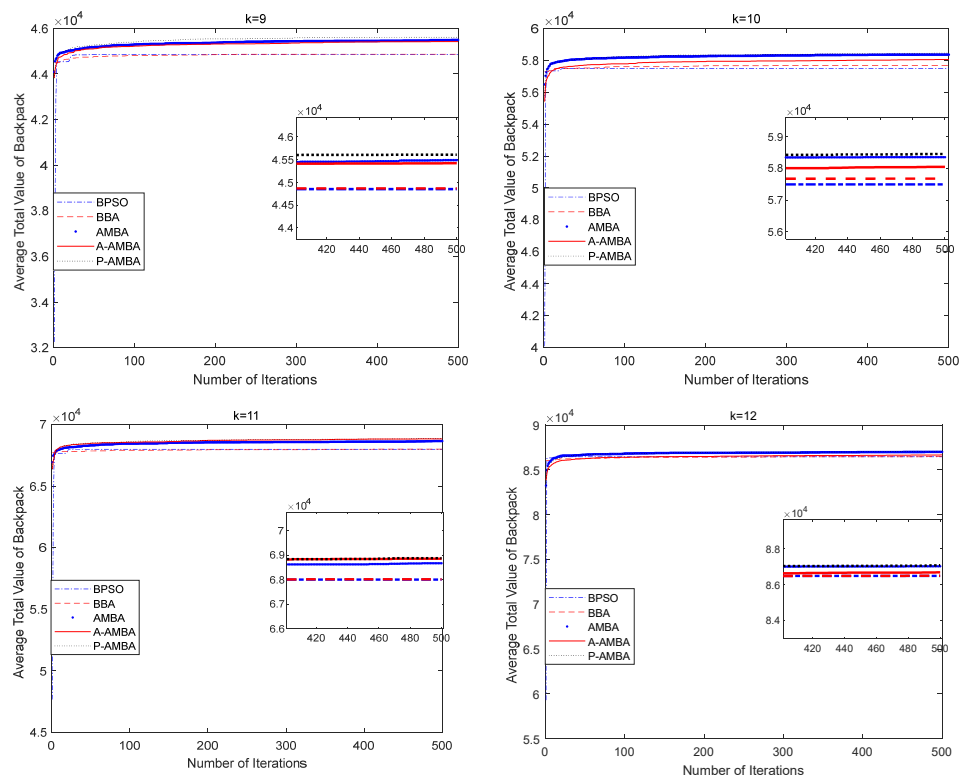
Figure 5. Average convergence curves of BPSO, BBA, AMBA, A-AMBA, and P-AMBA on some selected large-scale problems over 30 independent runs.
