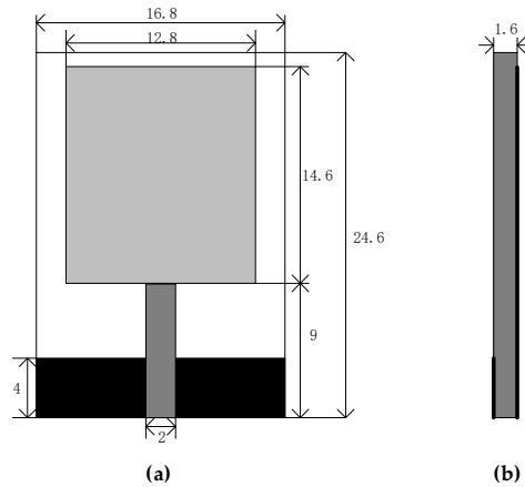
Figure 7. The top view (a) and the side view (b) of the initial antenna geometry (unit: mm).
