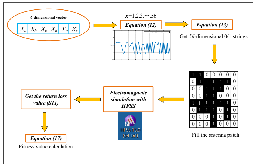
Figure 8. Schematic diagram of phase angle-modulated technology applied to antenna topology optimization.
