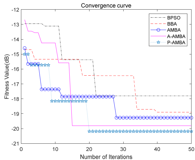
Figure 9. Comparison of the convergence curves of BPSO, BBA, AMBA, A-AMBA, and P-AMBA.
