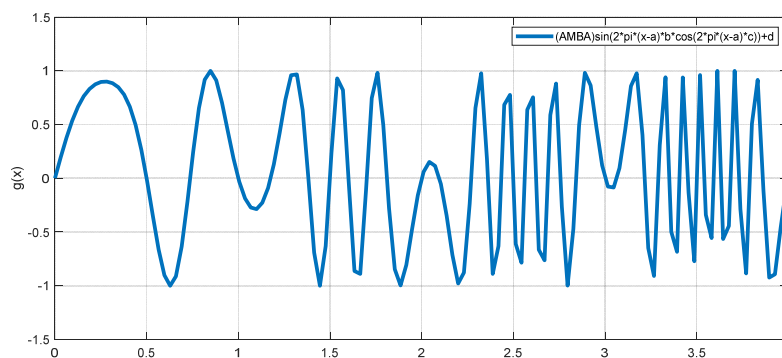
Figure 2. Generating function plotted with default values ( a = 0 , b = 1 , c = 0.5 , and d = 0 ).
