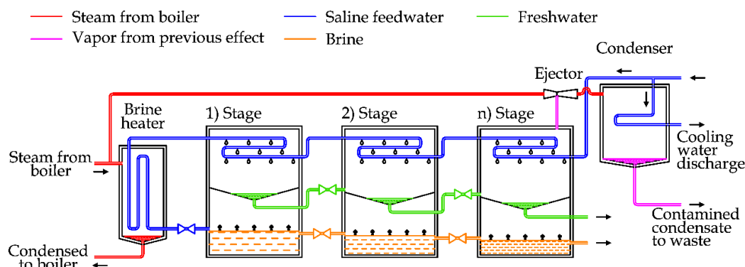
Figure 6. A schema of a Multi-Stages Flash (MSF) desalination unit.
