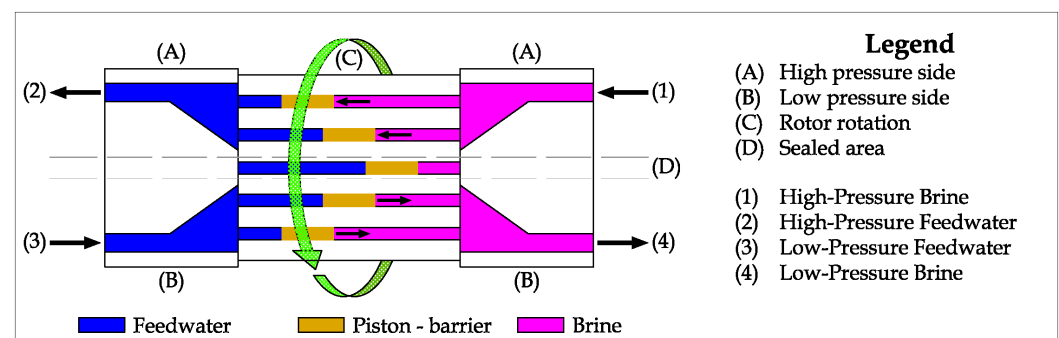
Figure 19. The working principles of a Rotary Pressure Exchanger.
