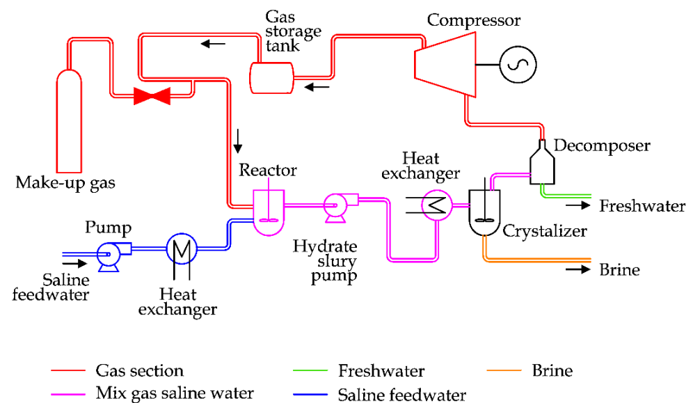
Figure 26. A schema of a Hydration desalination plant.
