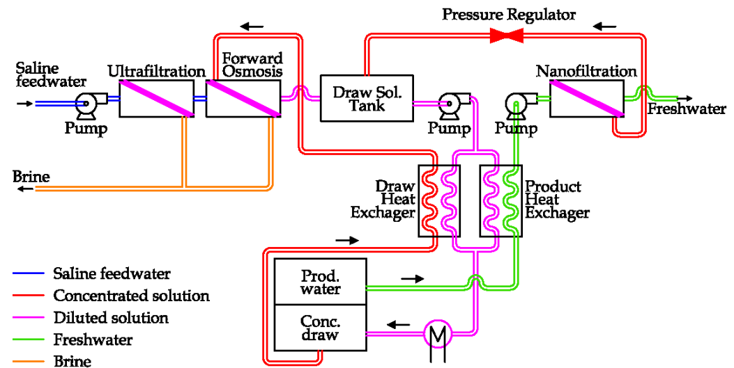
Figure 21. A schema of a Forward Osmosis desalination unit.
