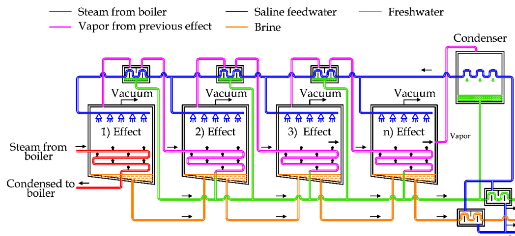
Figure 5. A schema of a Multi-Effect Distillation (MED) unit.
