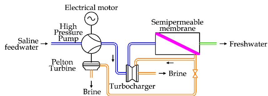
Figure 16. A schema of a RO unit with a Dual Turbine System.
