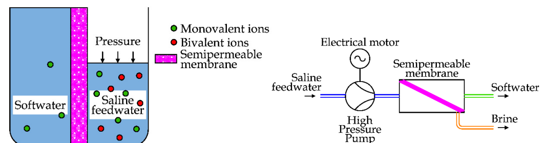
Figure 22. The working principles and schema of a nanofiltration unit.
