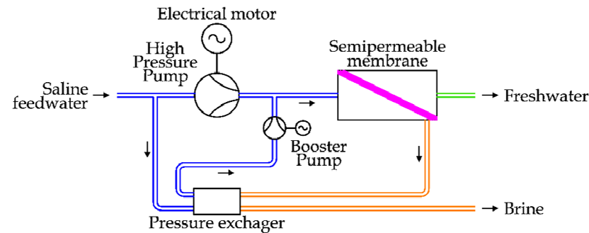
Figure 18. A schema of a RO unit with a Pressure Exchanger.
