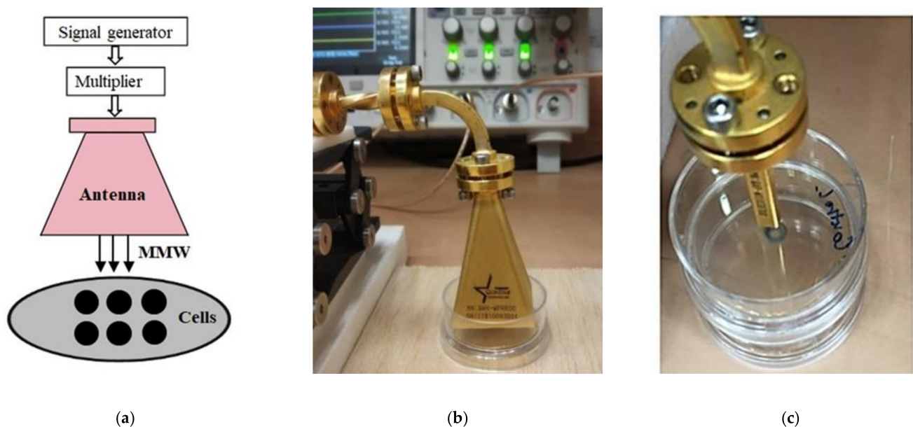
Figure 5. Block diagram of the experimental setup for irradiation and pictures of the pyramidal horn antenna and waveguide. (a) Schematic presentation of irradiating system. (b) Picture of a pyramidal antenna. (c) Picture of a waveguide.
