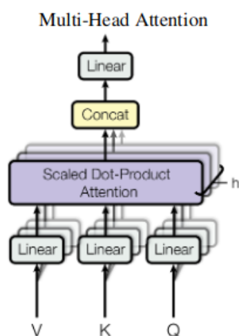
Figure 5. Multi-head Attention [24].
