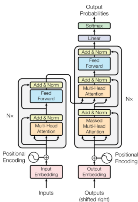
Figure 4. Transformer block architecture [24]. The left part is the encoder and the right part is the decoder.
