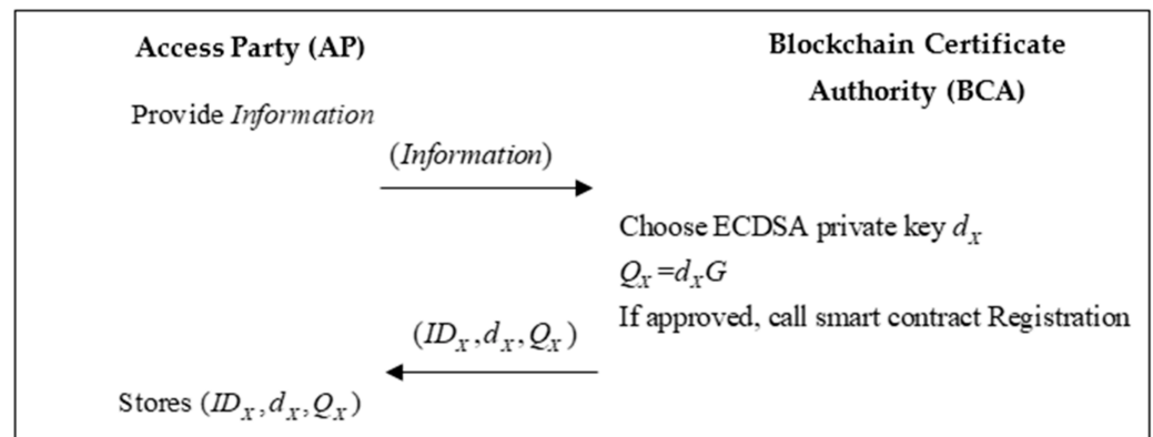
Figure 6. The flowchart of the registration phase.
