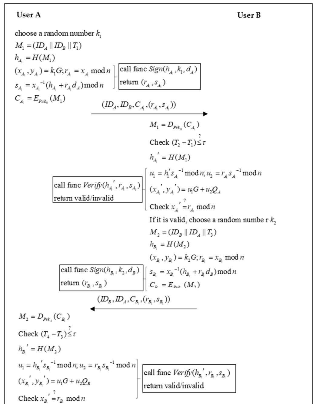
Figure 7. The flowchart of the authentication phase.
