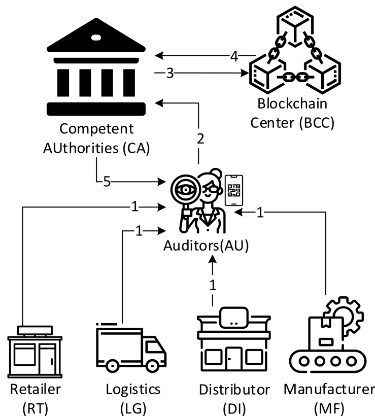
Figure 13. The audit mechanism in the verification phase.
