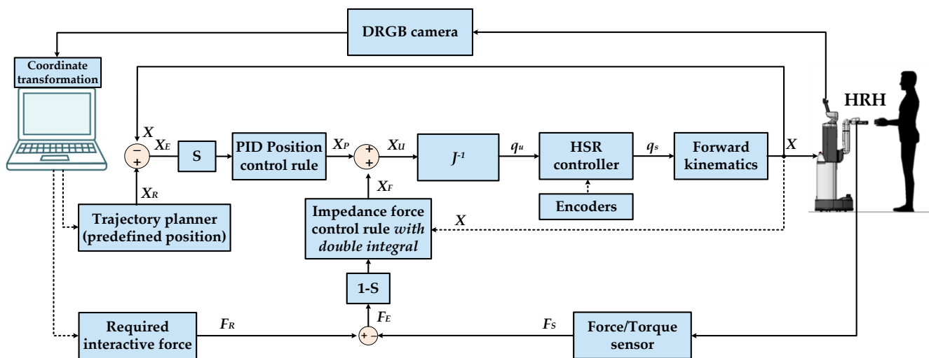
Figure 5. Hybrid PID position/impedance force control designed for the HSR in the HRH tasks.
