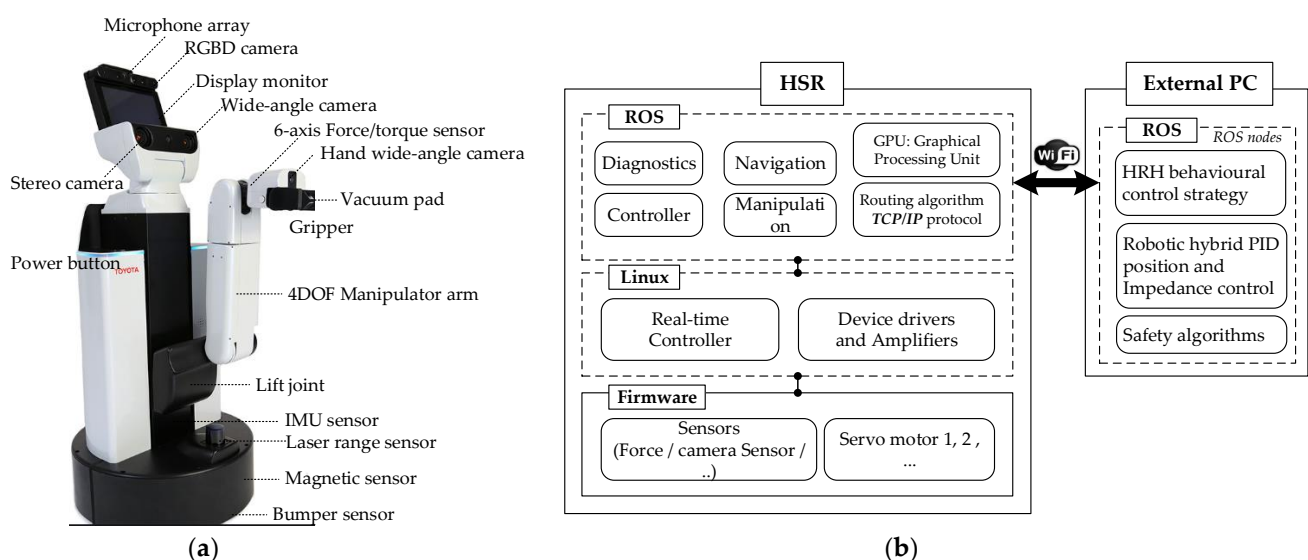
Figure 1. (a) The hardware equipment of the HRS and (b) HRS software architecture (connecting to an external PC).
