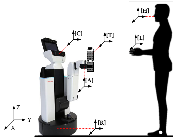
Figure 4. Reference frames of the HRH system.
