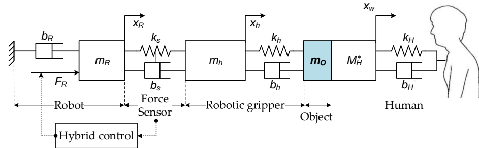
Figure 6. Mechanical schematic of the HRH based on a second-order-lumped-mass model.
