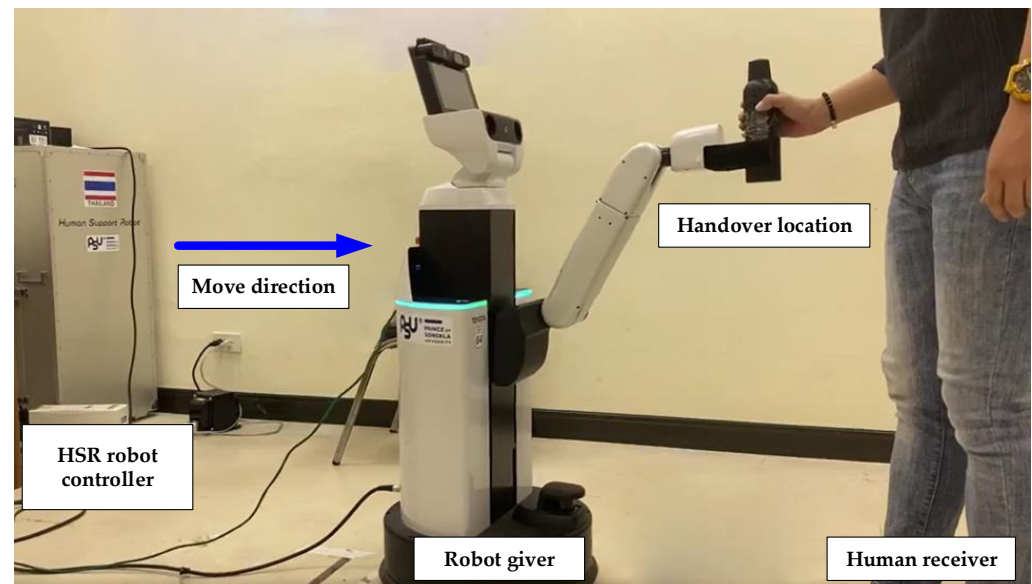
Figure 8. Experimental setup of the robot-to-human object handover system.
