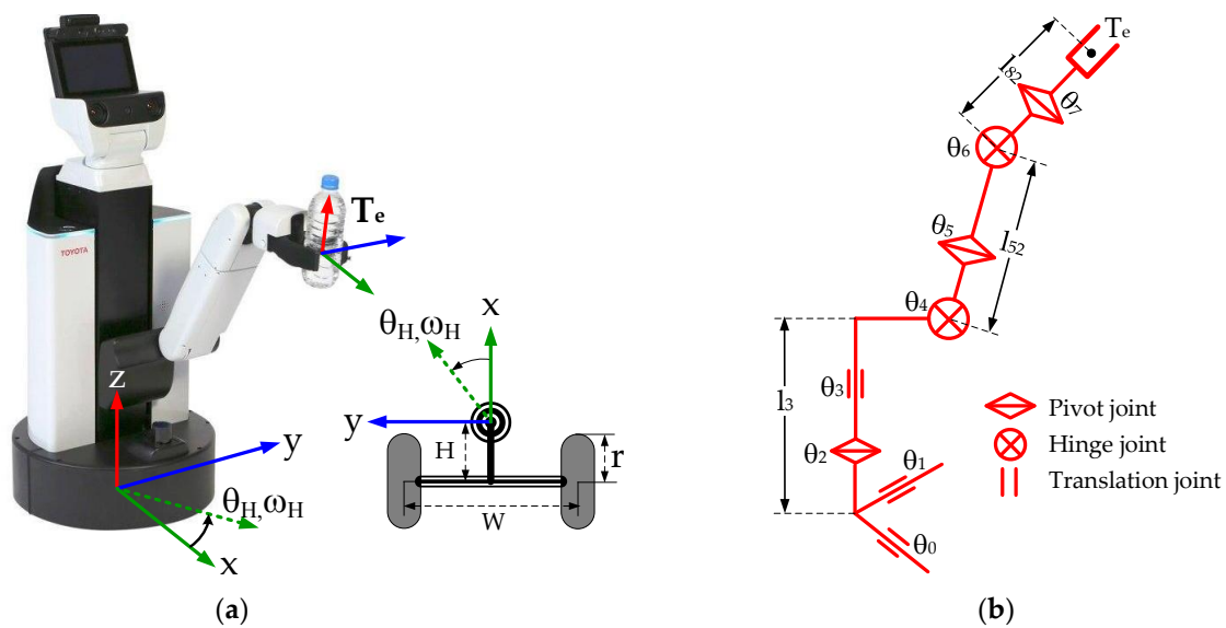
Figure 3. (a) The dual-wheel caster-drive robot base and (b) the robot joint configuration.
