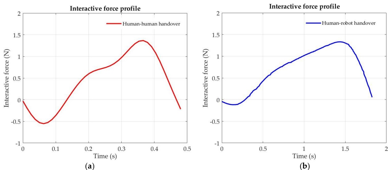
Figure 10. Interactive force profiles against the time of (a) the HHH test and (b) the HRH test.
