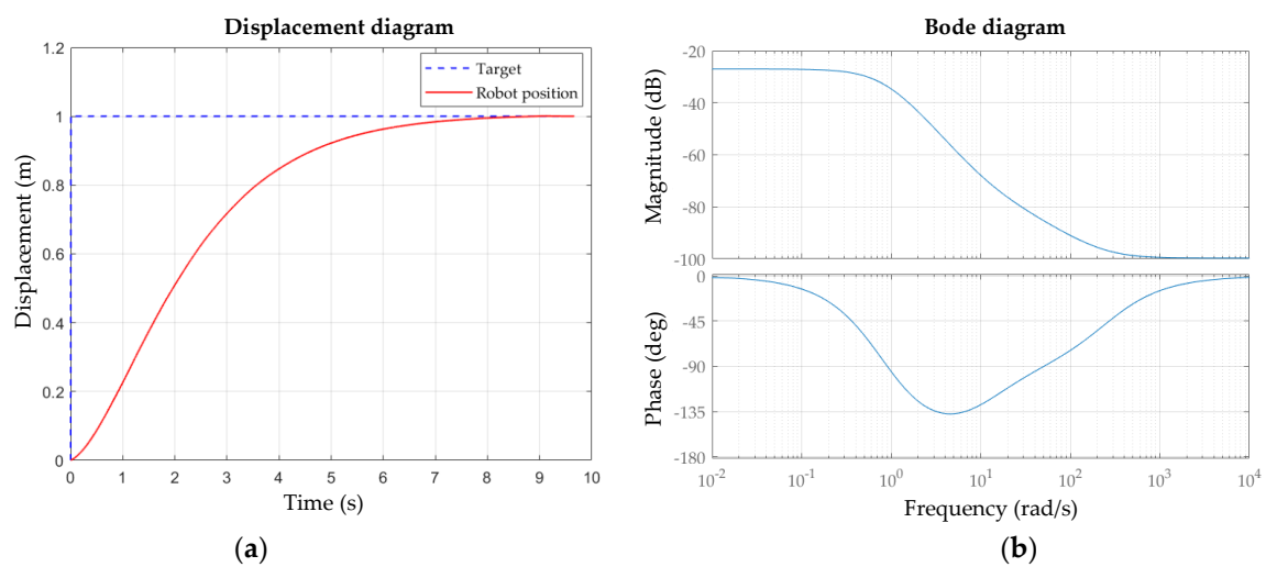
Figure 7. (a) Robot displacement profile in the HRH test and (b) Bode magnitude and phase plot.
