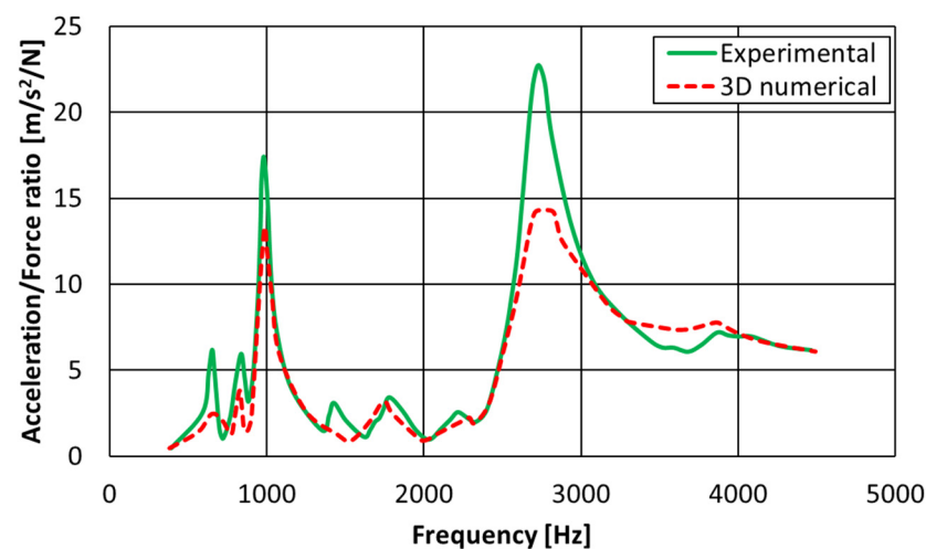
Figure 4. Experimental and numerical (“full 3D”) inertance vs. frequency measured at engine bracket, with excitation in the same point (highlighted in Figure 3a).
